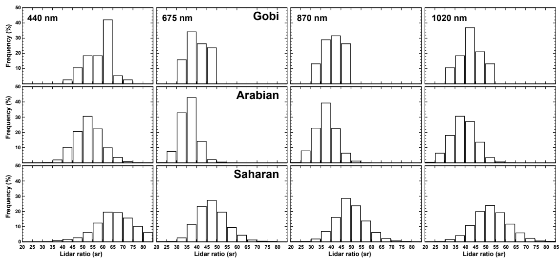
Figure 4. Same as Fig. 2 but for the dust lidar ratio S . Statistics for all regions are provided in Table 1.
