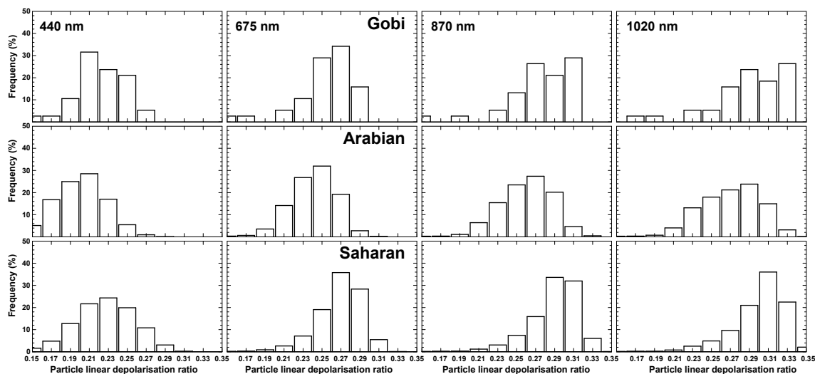
Figure 2. Frequency distribution of \delta for pure dust conditions. Rows refer to the Gobi, Arabian, and Saharan deserts, while columns refer to the wavelengths of 440, 675, 870, and 1020 nm, respectively. Due to the low number of pure dust cases, Great Basin ( N = 7 ) and Great Victoria ( N = 16 ) are not shown. Statistics for all regions are provided in Table 1.
