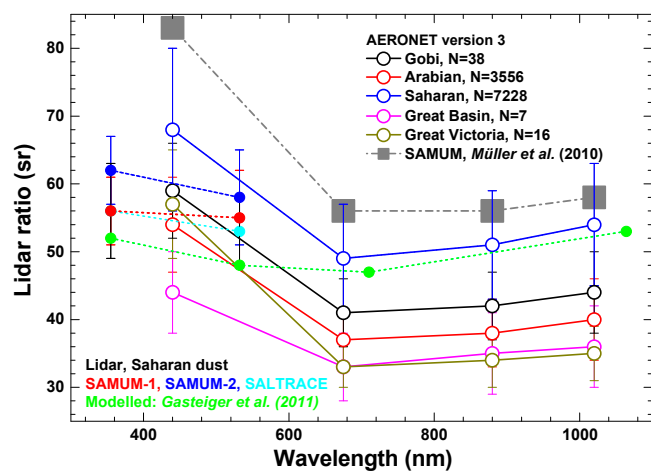
Figure 5. Spectral variation of S as derived from AERONET observations for pure dust (open symbols) compared to published values (solid symbols) from two-wavelength lidar observations of Saharan dust during its transport over the Atlantic (SAMUM-1, Tesche et al., 2009a; SAMUM-2, Tesche et al., 2011; SALTRACE, Groß et al., 2015) and the results of light-scattering modelling (Gasteiger et al., 2011). The gray line and symbols present the AERONET-derived S from the comparison study for Saharan dust of Müller et al. (2010).
