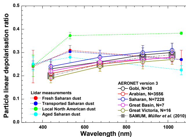
Figure 3. Spectral variation of \delta as derived from AERONET observations for pure dust (open symbols) compared to published values from triple-wavelength lidar observations (solid symbols) of fresh Saharan dust close to the source (Freudenthaler et al., 2009), transported Saharan dust and local North American dust (Burton et al., 2015), and aged Saharan dust after one week of transport (Haarig et al., 2017). The gray line and symbols present the AERONET-derived \delta from the comparison study for Saharan dust of Müller et al. (2010).
