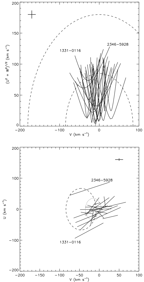
Fig. 12.— The kinematics of the sample. Top panel: Toomre diagram. The solid lines represent the velocity ranges of each brown dwarf, obtained assuming a radial velocity range of -100/+100 \text{ km s}^{-1} . The dashed circles are the boundary between thin disk and thick disk stars (inner circle) and between thick disk and halo stars (outer circle), as used by Nissen (2004). Bottom panel: U - V plot showing the velocity ranges obtained for our targets. Overplotted for reference are the velocity ellipsoids obtained by Bensby et al. (2003) for thin disk (dotted) and thick disk (dashed) respectively. In each plot the outliers are labelled. Typical uncertainties are shown in the top-left and top-right corner, respectively.
