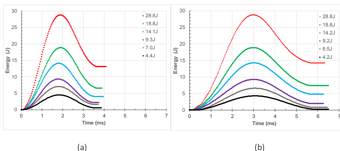
Fig. 7 Energy - time curves of (a) woven carbon fibre composite laminates and (b) woven glass fibre composite laminates
