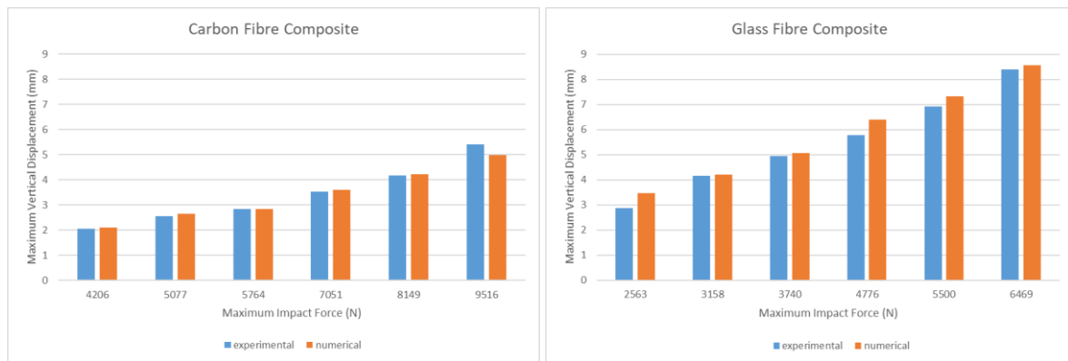
Fig. 4 Comparison of the experimental and theoretical maximum deflection of a) carbon fibre samples and b) glass fibre samples.
