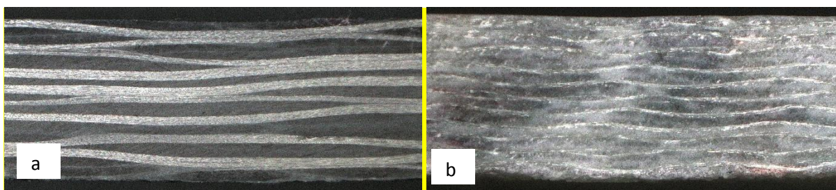
Fig. 3 Cross section to show the indentation of a) carbon fibre sample tested at 10 J and b) glass fibre sample tested at 5 J.
