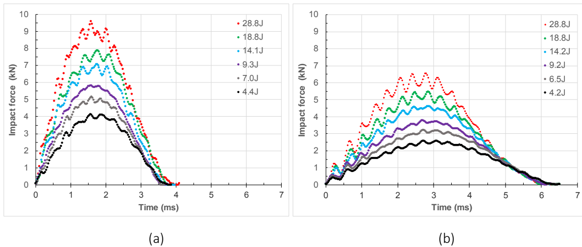
Fig. 2 Impact force – time curves of (a) woven carbon fibre composite laminates and (b) woven glass fibre composite laminates
