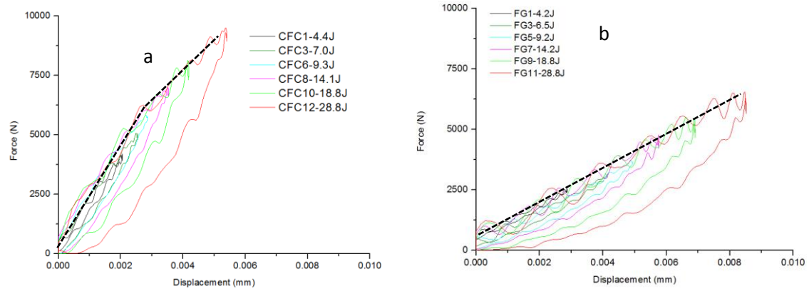
Fig. 5 Impact force – displacement curves of a) woven carbon fibre composite laminates and b) woven glass fibre composite laminates. Dotted lines show the change in stiffness observed for the carbon fibre composite.
