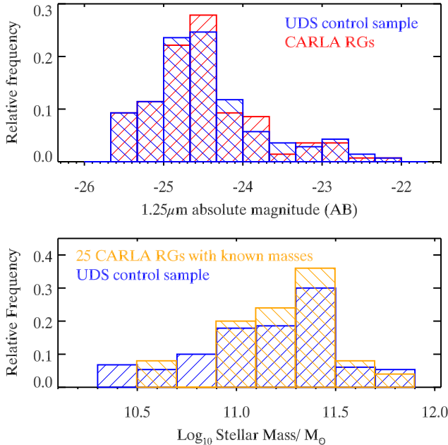
Figure 2. A comparison of the rest-frame 1.25\mu\text{m} absolute magnitudes (top panel) and stellar masses (bottom panel) between the CARLA RLAGN and the control galaxies. There is no significant difference in the rest-frame 1.25\mu\text{m} absolute magnitudes, and the stellar masses of the control galaxies are very similar to the stellar masses of the 25 CARLA RLAGN that were measured using SED fitting of 3.6 to 70\mu\text{m} photometry by Seymour et al. (2007). Hence the control galaxies are well-matched in stellar mass to the CARLA RLAGN.
