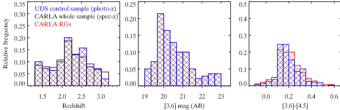
Figure 1. The distributions of the redshifts (left), [3.6] magnitudes (middle), and [3.6]-[4.5] colours (right) of the CARLA reduced radio galaxy sample (red), the UDS control sample (blue) and the whole CARLA sample (black; shown in the left panel only as the IRAC magnitudes and colours of the RLQs are dominated by the quasar light. See Section 2.2.1 for details). The control sample is closely matched to the CARLA radio galaxy sample; KS tests result in probabilities in the range of 0.3-0.97, so there are no significant differences between these distributions.
