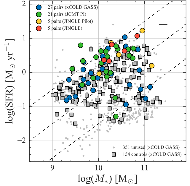
Figure 3. Global star formation rate versus stellar mass relation of galaxies discussed in this work. Galaxies in pairs used in this work are shown as colored symbols. Galaxies from the control sample are shown as gray squares. Those in the xCOLD GASS sample that are not used in the analysis are shown as gray dots (see text for details). SFR and M_* values are taken from the MPA-JHU catalog. From top to bottom, the three dashed lines correspond to \log(\text{sSFR}/\text{yr}^{-1}) = -9.5, -10.5, \text{ and } -11.5 , respectively.
