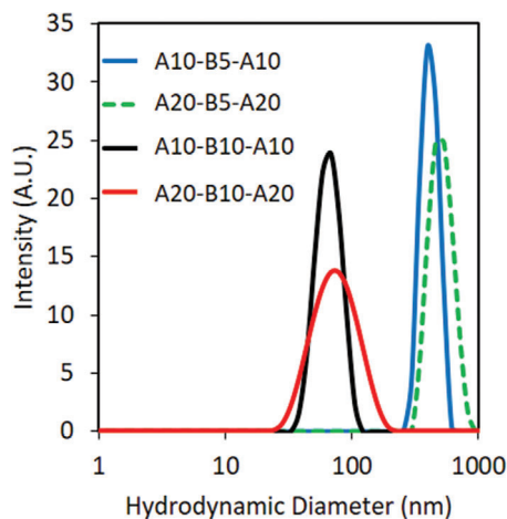
Figure 3. Block copolymer aggregate size distributions in dilute aqueous solutions ( 1 \text{ mg mL}^{-1} ) at 50 \text{ }^\circ\text{C} as determined by DLS.
