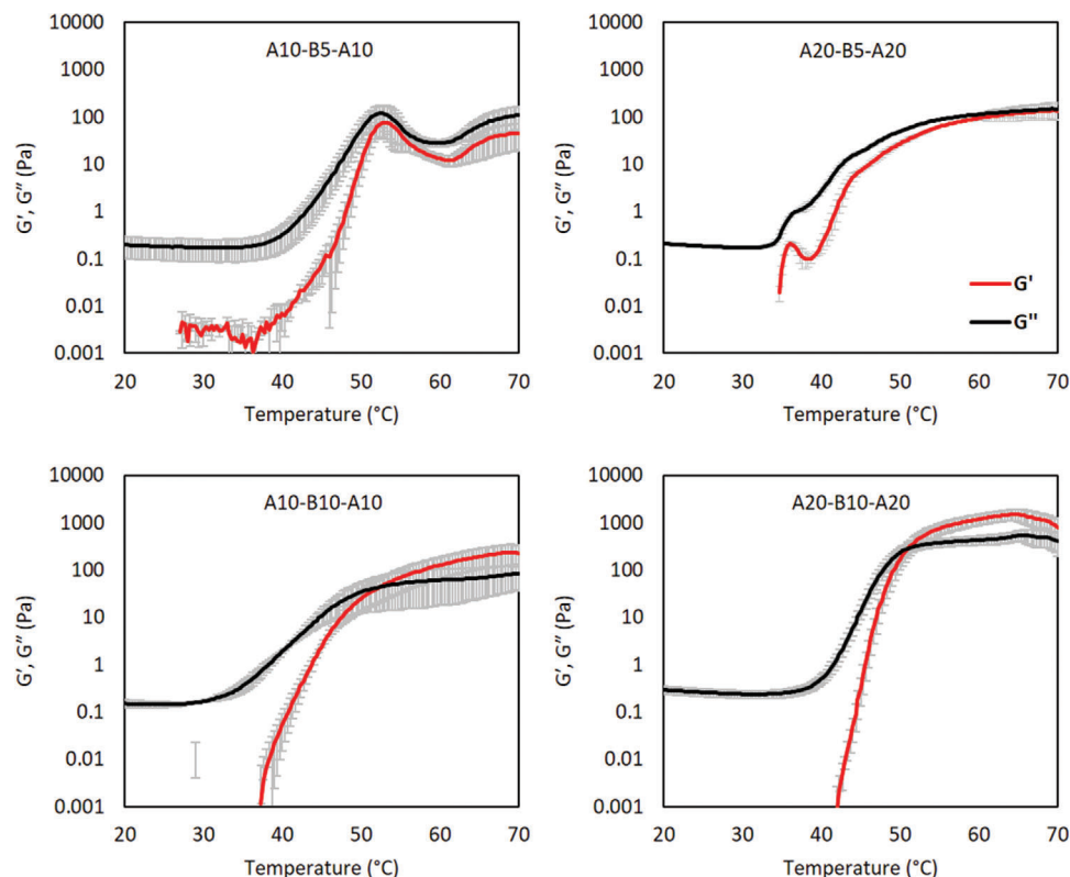
Figure 2. PDEA- b -PEG- b -PDEA copolymer solutions (20% (w/v)) studied by small-amplitude oscillatory shear rheology as a function of temperature, measured at a shear stress of 1 Pa and a frequency of 1 Hz.
