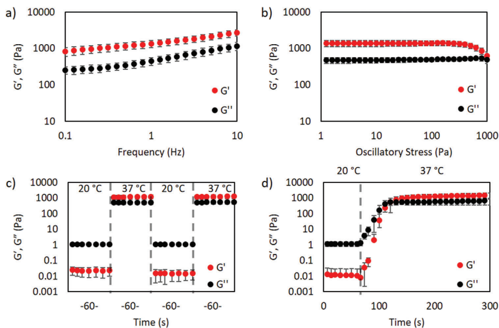
Figure 8. Rheological evaluation of the optimized A20-B10-A20 PDEA-b-PEG-b-PDEA copolymer as a 30% (w/v) solution in 0.3 M NaCl. a) Frequency and b) amplitude sweeps at 37 °C. c) Reversibility of gelation determined by small-amplitude oscillatory rheology with switching between sol (20 °C) and gel (37 °C) states (please note there was a 120 s equilibration time at each temperature change during which data was not collected). d) Time taken for gelation to occur determined by holding at 20 °C for 60 s, then switching to 37 °C.
