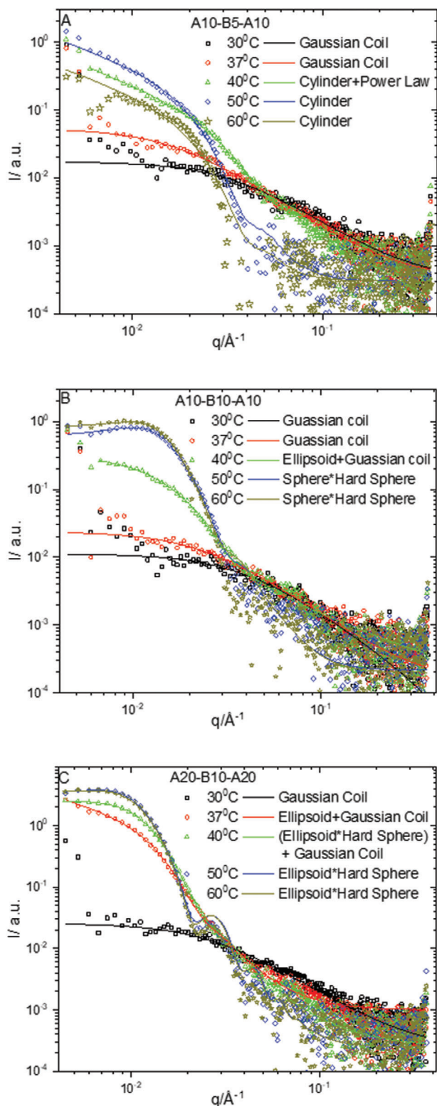
Figure 4. SAXS profiles of a) A10-B5-A10, b) A10-B10-A10, and c) A20-B10-A20 PDEA-b-PEG-b-PDEA copolymers at 5 wt% over the temperature range 30 to 60 °C.
