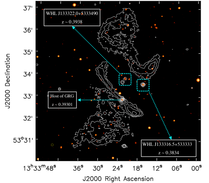
Fig. 6. GRG J133322.79+533250.94 possibly amidst galaxy cluster relics. The background image in an orange colour is SDSS I band optical image, which is superimposed with LoTSS DR1 high-resolution ( 6'' ) contours.
