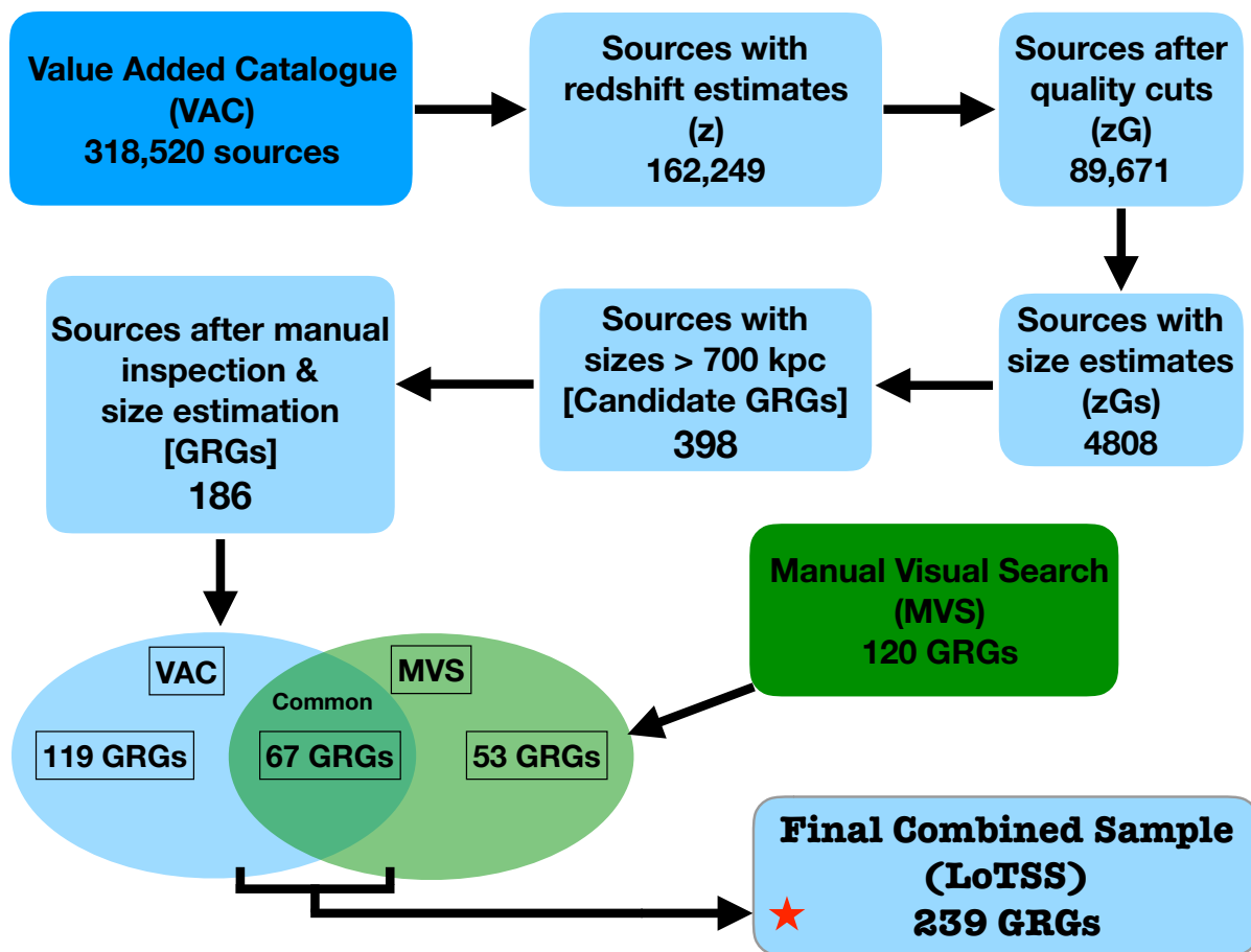
Fig. 2. Above figure shows schematics for finding GRGs from LoTSS DR1, using VAC and MVS in steps. More details are presented in Sect. 2.
