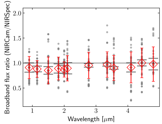
Fig. C.1. Ratio of apodised broad-band fluxes extracted from the projected MSA shutter regions on the NIRCcam imaging compared to fluxes obtained from convolving PRISM/CLEAR spectra with the NIRCcam filter transmission curves. Refer to the text for more details. Grey points show values derived for each independent pointing of each galaxy targeted in this work. Horizontal grey marks indicate the typical 1\text{-}\sigma measurement uncertainty on the individual measurements in each filter (which encompasses uncertainties from both NIRCcam and NIRSspec). Red diamonds and errorbars show the median and standard deviation for each filter.
