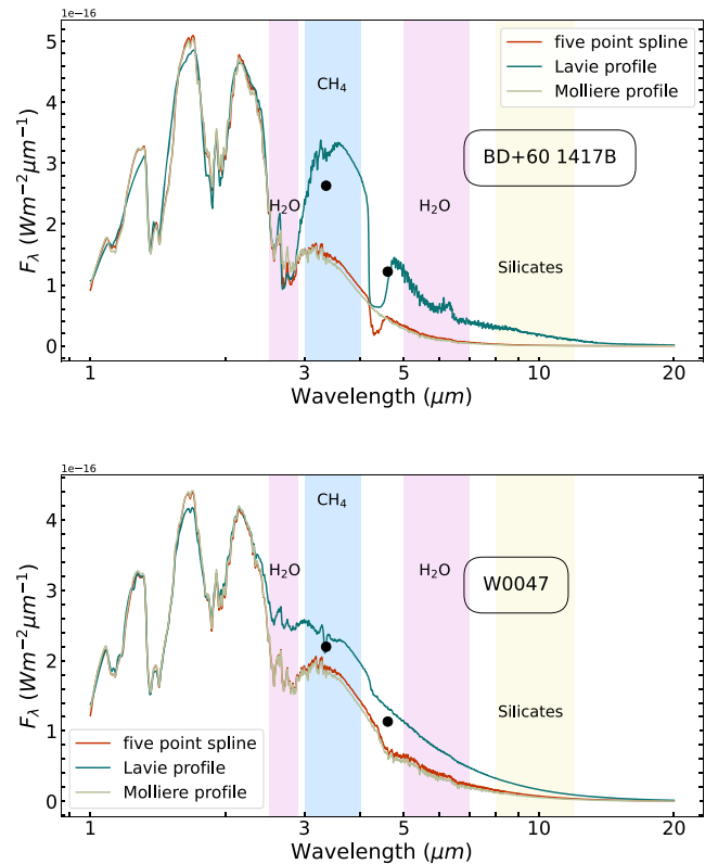
Figure 11. Extracted mid-infrared spectra for BD+60 1417B and W0047 with important molecular gases highlighted.
