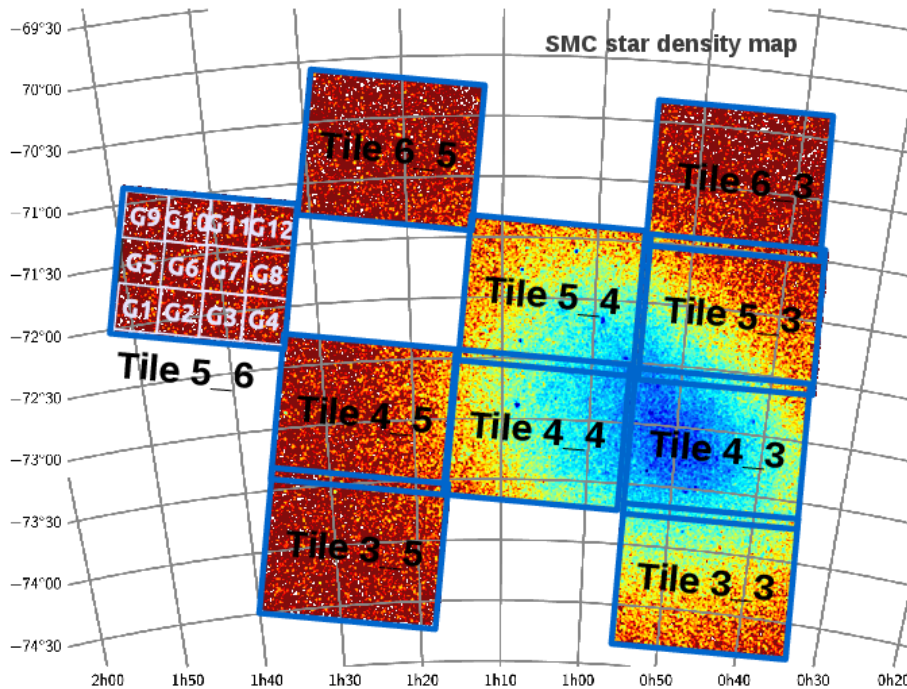
Figure 1. Sky position of all tiles analysed in this work, as listed in Table 1. Each tile is subdivided into 12 small subregions, as illustrated here for the tile 5.6. The plot includes only the tiles with a high fraction of the planned VMC observations already completed; the complete, final coverage of the SMC by the VMC survey can be appreciated in Cioni et al. (2011).
