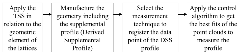
Fig. 4 The workflow of the TSS mechanism for tolerancing lattice structure [43, 44]
