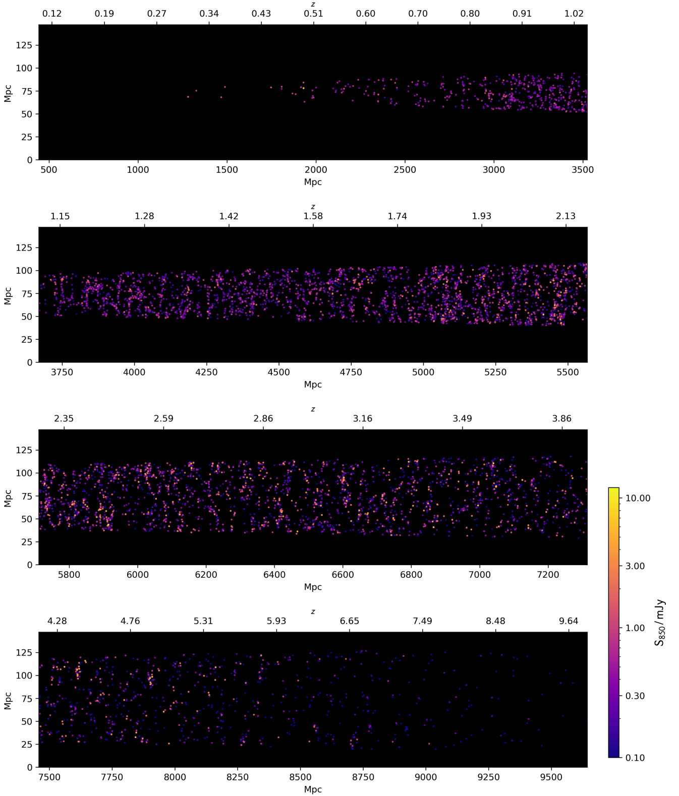
Figure 3. SIMBA reconstructed lightcone over 0.5 \text{ deg}^2 , between 0.1 < z < 10 . Each point shows a galaxy coloured by 850 \mu\text{m} flux density. The radial distance on the x -axis is the comoving distance. The transverse distance d on the y -axis is the comoving distance, and is d = [42.6, 67.0, 80.4, 91.2, 103.72, 116.3] at z = [1, 2, 3, 4, 6, 9] , respectively.
