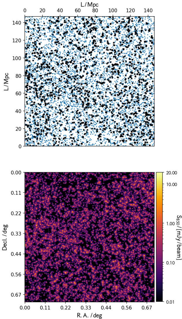
Figure 4. Top: map of a single lightcone realisation using all selected objects ( \text{SFR}_{\text{inst}} > 20 M_{\odot} \text{yr}^{-1} ) on the sky plane (blue points). Sources blended along the line of sight are shown by black crosses. Bottom: The 850 \mu\text{m} map convolved with the SCUBA-2 beam (Dempsey et al. 2013), coloured by flux density.
