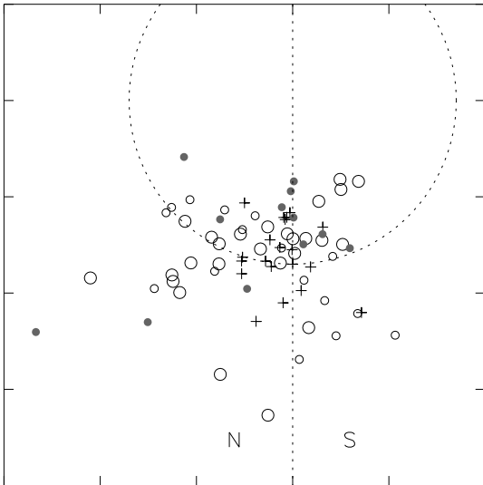
Figure 6: The galactic disk distribution of warm-dust PNe on a face-on view of the disk, with distances from Zhang (1995). Ticks are every 5 kpc, and the solar circle is shown in dashed line.
