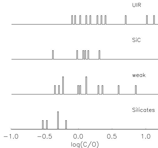
Figure 2: Histogram showing the number of nebulae of each dust types as a function of gas phase C/O ratios. Typical error bars are \sim +0.11/-0.15 horizontally for a 20 per cent uncertainty in the abundance calculations.
