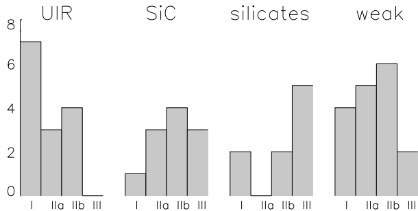
Figure 3: Relative proportion of PN dust types among Peimbert (1978) types, with sub-types from Faúndez-Abans & Maciel (1987).
