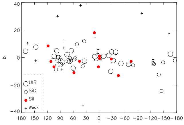
Figure 4: Sky distribution of PN dust types.
