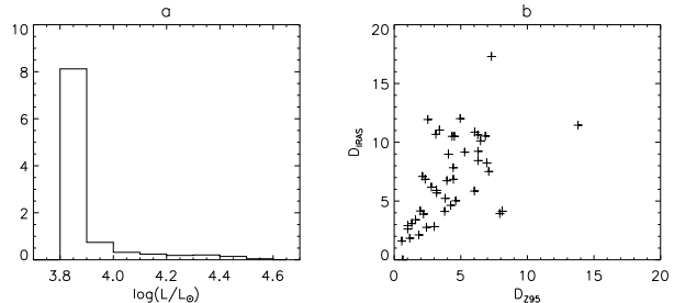
Figure 5: a) Synthetic PN luminosity function from the initial-final mass relationship of Groenewegen & de Jong (1993), and with progenitor ZAMS masses between 1.2 and 7 M_{\odot} . b) The relationship between D_{IRAS} and Zhang (1995) for the PNe with warm dust emission.
