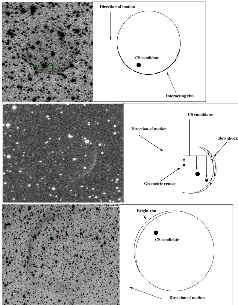
Figure 4: Examples of WZO2 types. Top: Size=1.2 arcmin and SB=3.4e^{-17} erg cm ^{-2} s ^{-1} arcsec ^{-2} . Middle: Size= 8.5 arcmin and SB=1.1e^{-16} erg cm ^{-2} s ^{-1} arcsec ^{-2} , Bottom: 4.3 arcmin and SB=2.7e^{-16} erg cm ^{-2} s ^{-1} arcsec ^{-2} . North on the top and East on the left.
