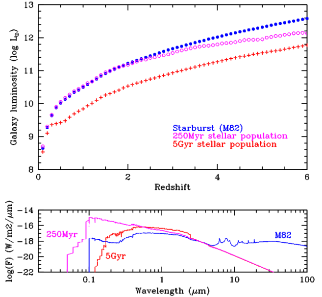
FIG. 17.— Top panel : SERVS faintest galaxy to be detected, in units of solar luminosities (integrated luminosity from the optical to the far-IR: 0.1\mu\text{m} –1 mm) at a given redshift. Three Spectral Energy Distribution (SED) models are considered here and shown in the bottom panel . The three SEDs consist of an M82-like starburst galaxy (in blue), a 250 Myr stellar population (magenta) and a 5 Gyr stellar population (red), scaled to the same 3.6\mu\text{m} rest-frame. SERVS can detect L^* galaxies out to z \sim 4 , and 0.1L^* out to z \sim 1 . At redshift 5, a starburst galaxy of luminosity \sim 10^{12} L_{\odot} could potentially be detected.
