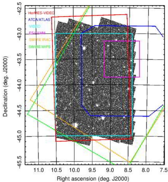
FIG. 3.— The [3.6] SERVS mosaic image of the ES1 field. Surveys of comparable size are shown here, such as the HerMES-VIDEO field ( in red ), the ATCA/ATLAS radio survey ( dark blue ), the VIDEO survey ( light blue ), the deep ES1-XMM field of Feruglio et al. (2008) ( magenta ), SWIRE IRAC ( dashed orange ) and SWIRE MIPS ( dashed green ). Surveys encompassing the entire field such as HerMES Level 6 are not shown here. More details about ancillary data coverage can be found in Section 5.
