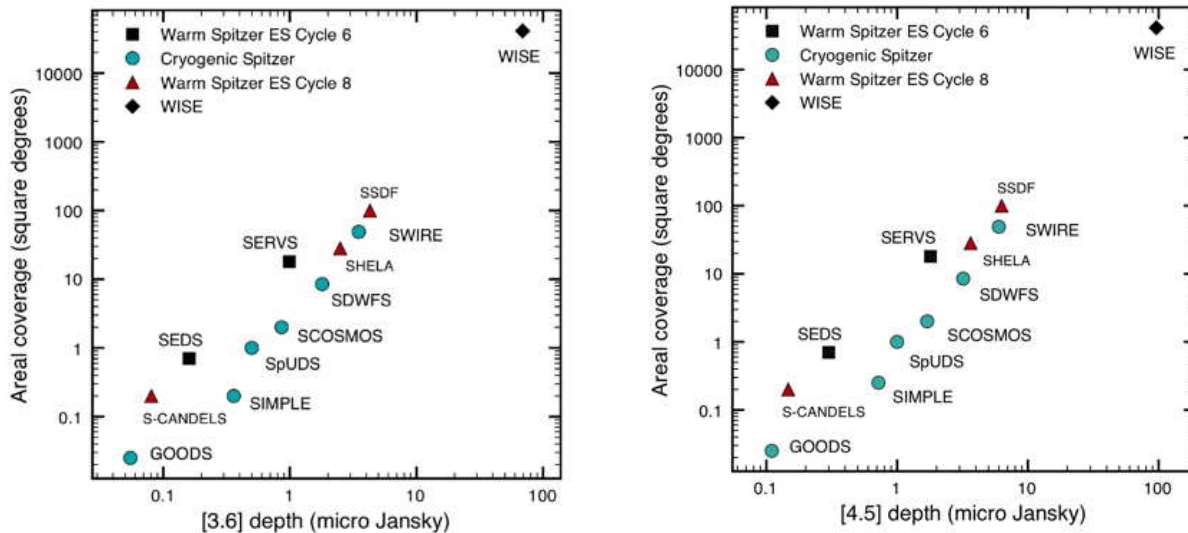
FIG. 1.— Area versus depth for SERVS compared to other surveys at wavelengths of \approx 3.6\mu\text{m} ( left panel ) and \approx 4.5\mu\text{m} ( right panel ). For consistency, the depth shown is the 5\sigma limiting flux for point sources, excluding confusion noise ( \sigma_{\text{pp}} as described in Section 4.2), calculated from the Spitzer performance estimation tool ( http://ssc.spitzer.caltech.edu/warmmission/propkit/pet/senspet/index.html ) in each case. The surveys are ( from left to right ): GOODS, the Spitzer follow-up to the CANDELS HST survey (Cosmic Assembly Near-IR Deep Extragalactic Legacy Survey, Grogin et al. 2011; Koekemoer et al. 2011), the Spitzer Extragalactic Deep Survey (SEDS, Program identifier - hereafter PID - 60022, 61040, 61041, 61042, 61043, P.I. G. Fazio), the Spitzer IRAC/MUSYC Public Legacy in E-CDFS (SIMPLE) survey ( Spitzer , PID 20708), the Spitzer Ultra Deep Survey (SpUDS, PID 40021, P.I. J.S. Dunlop), S-COSMOS, the Spitzer Deep Wide-Field Survey (SDWFS, Ashby et al. 2009), the Spitzer -HETDEX Exploratory Large Area (SHELA, PID 80100, P.I. C. Papovich) Survey, SWIRE, the SPT- Spitzer Deep Field (SSDF, PID 80096, P.I. S. Stanford) and the Wide-Field Infrared Explorer (WISE, Wright et al. 2010).
