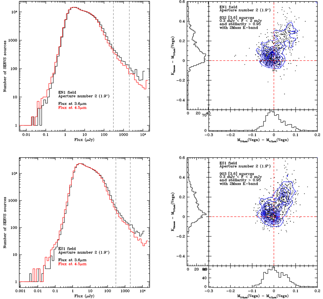
FIG. A.1.— Left side: SERVS number counts versus flux at [3.6] and [4.5] for the EN1 ( top ) and ES1 ( bottom ) fields. Grey dashed lines show the selection of sources used in the bottom plot (with fluxes as 0.3 < f < 2 \text{ mJy} ). Right side: Color-color plot showing K_{2\text{MASS}} - M_{3.6\mu\text{m}}(\text{Vega}) versus M_{3.6\mu\text{m}}(\text{Vega}) - M_{4.5\mu\text{m}}(\text{Vega}) for sources within the flux range defined by the grey dashed lines above, plus a cut in stellarity index > 0.95 and the existence of a 2MASS K-band measurement as an additional constraint. Red dashed lines help pinpoint the location of the (0,0) point in this diagram.
