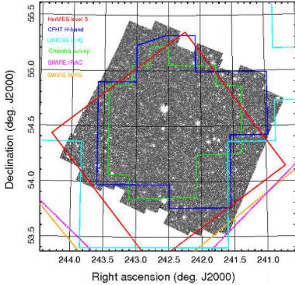
FIG. 2.— The [3.6] SERVS mosaic image of the EN1 field. Surveys of comparable size are shown here, such as HerMES level 5 ( in red , see Oliver et al. 2012 for details), CFHT H-band ( dark blue ), UKIDSS J & K-bands ( light blue ), the Chandra X-ray survey ( green ), SWIRE IRAC ( dashed magenta ) and SWIRE MIPS ( dashed orange ). Surveys encompassing the entire SERVS field such as HerMES Level 6 and the GMRT survey at 610 MHz are not shown here. More details about ancillary data coverage can be found in Section 5.
