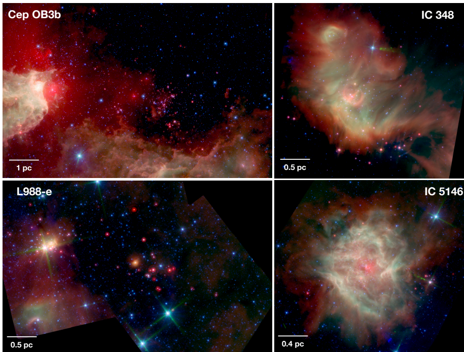
Fig. 1 Three-color Spitzer images (3.6 (blue), 5.8 (green), and 24\ \mu\text{m} (red)) of young, nearby ( d < 1000\ \text{pc} ) clusters. Cluster source catalogs are contained in the Spitzer Extended Solar Neighbourhood Archive (SESNA, Gutermuth et al. in prep). Top left: Young (4-5 Myr), massive cluster Cep OB3b, which is part of the Cep OB3 molecular cloud complex (Gutermuth et al., 2011; Allen et al., 2012). Top right: IC 348 cluster (2-3 Myr), which is forming in a sub-region of the Perseus molecular cloud (Gutermuth et al., 2009). Bottom left: Extended field containing exposed cluster L988-e (courtesy of R. Gutermuth). Bottom right: Small, dense cluster IC 5146, where protostars are forming around a bright PAH emission bubble (Gutermuth et al., 2009).
