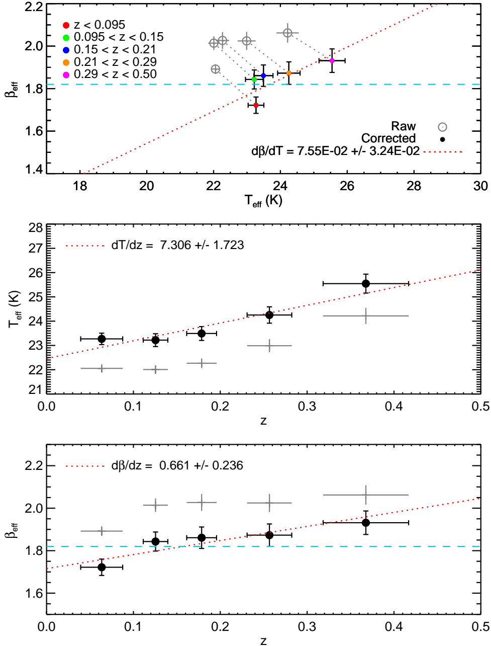
Figure 12. Top: Comparison between the values derived using our method for T_{\text{eff}} and \beta in bins of redshift, such that there are approximately equal numbers of galaxies in each bin. Middle: Variation between the recovered T_{\text{eff}} as a function of redshift, showing a > 4\sigma positive correlation. Bottom: recovered \beta as a function of redshift, showing only weak evidence for redshift dependence of emissivity index in H-ATLAS. The median \log_{10}(L_{\text{dust}}/L_{\odot}) for each redshift bin is 10.01, 10.42, 10.67, 10.97 and 11.31, from the lowest to the highest redshift bin, respectively.
