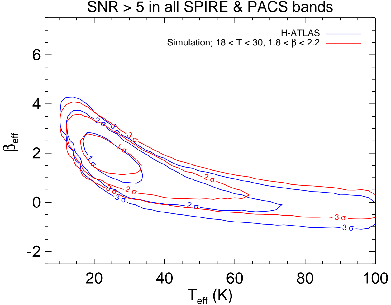
Figure 7. Comparison between the 2D confidence intervals for T_{\text{eff}} and \beta_{\text{eff}} shown for the subset of the H-ATLAS catalogue detected at \geq 5\sigma in all PACS/SPIRE bands (in blue) and for a similar subset of our simulation (in red), with the input values of temperature and emissivity truncated relative to the full simulation, as discussed in the text. The values input to our simulation for T_{\text{eff}} and \beta_{\text{eff}} have no intrinsic correlation.
