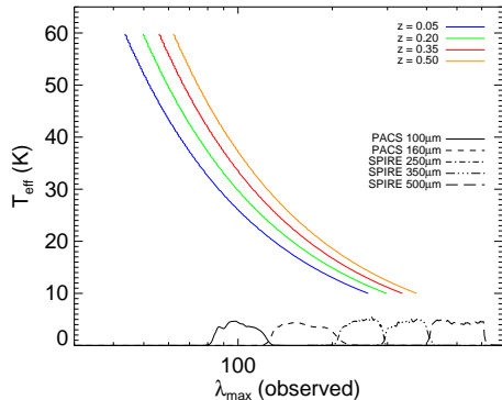
Figure 15. The relationship between the wavelength of the peak in the dust SED and the modified black-body-equivalent temperature for redshifts spanning our sample ( z = 0.05, 0.20, 0.35 and 0.50 ), assuming \beta = 1.82 . The PACS (100 and 160 \mu\text{m} ) and SPIRE (250, 350 & 500 \mu\text{m} ), response curves are overlaid for the purposes of comparison.
