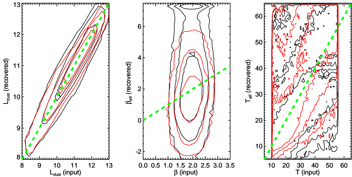
Figure 3. Comparisons between the input values for L_{\text{dust}} , \beta and T_{\text{eff}} (left, centre and right-hand panels, respectively) and their median-likelihood (red) or best-fit (black) estimates in our H -ATLAS-like simulation. The contour levels correspond to the regions enclosing 68.3, 95.5 and 99.7 per cent of the recovered values. The green dashed lines indicate the ideal relation between input and recovered values, and the excess of best-fit sources around \beta_{\text{eff}}(\text{recovered}) \approx 7.5 in the centre panel results from the tendency of best-fit values to accumulate where the posterior probability distribution is truncated by the bounds of the prior.
