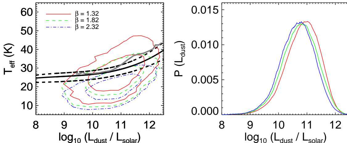
Figure 18. Left: The effects of choosing different values of emissivity index on the derived values of T_{\text{eff}} and L_{\text{dust}} using our simple fixed- \beta SED fitting code on the H -ATLAS phase 1 data set. The distribution of the values derived assuming \beta = 1.32 , 1.82 and 2.32 are shown as the red, green and blue contours respectively, with the best-fit relationships from Chapman et al. (2003) and Hwang et al. (2010) overlaid in black and grey, respectively. The contour levels show the regions enclosed by 68.3 and 95.5 per cent of the data at each value of \beta . Right: stacked PDFs of L_{\text{dust}} recovered using the same three values and in the same colour scheme.
