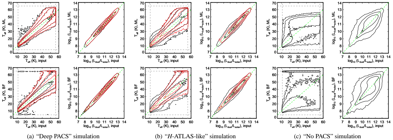
Figure 14. The results of comparing the input and output values for temperature and dust luminosity in our fixed \beta = 1.82 , “Deep PACS” (a), “ H-ATLAS -like” (b) and “no PACS” (c) simulations, from left to right. The top row shows the median-likelihood values for each parameter, while the bottom row shows the best-fit values, with the thick black contours indicating the regions that bound 68.3, 95.5 and 99.7 per cent of the full set of simulated sources, and the thin red contours showing the same percentiles for the \geq 5\sigma PACS-detected fraction of sources. The dashed green lines indicate equal input and output values, while the grey dashed lines in the temperature plots indicate the bounds of the input and output prior distribution; 11 < T_{\text{eff}} < 56 K and 5 < T_{\text{eff}} < 65 K, respectively.
