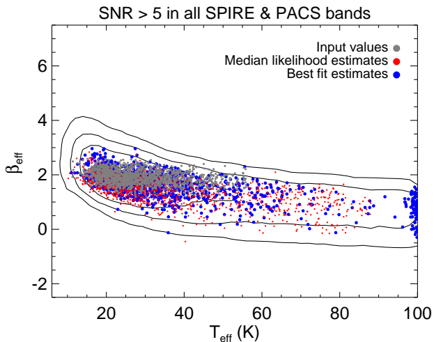
Figure 5. Comparison between the values of temperature and emissivity index input to our simulation (grey points) and derived using best-fit (blue) and medium-likelihood (red) estimators. The clump of blue points reflects the tendency for best-fit values to be returned on the bounds of the temperature prior when the prior truncates the PDF. In contrast to figure 4, this plot shows only sources with \geq 5\sigma detections in each PACS/SPIRE band.
