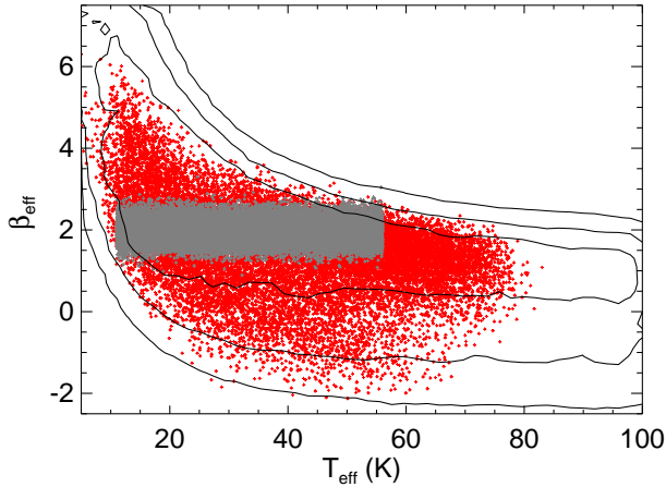
Figure 4. Two dimensional stacked probability density function for T_{\text{eff}} and \beta shown by the solid black contours indicating the regions enclosing 68.3, 95.5 and 99.7 percent of the PDF. The median-likelihood estimates for each simulated galaxy well-described by our model are shown as the red points with the overlaid grey points indicating the input values, revealing the extent of the artificial anti-correlation.
