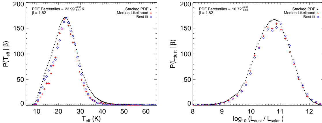
Figure 17. Left: The stacked PDF of \beta = 1.82 isothermal temperature for 250 \mu\text{m} -selected galaxies in H -ATLAS (black crosses) with the median-likelihood and best-fit estimates overlaid as the red crosses and blue diamonds, respectively. Right: Stacked PDF for L_{\text{dust}} and histogram of median-likelihood and best-fit values in the same colour scheme.
