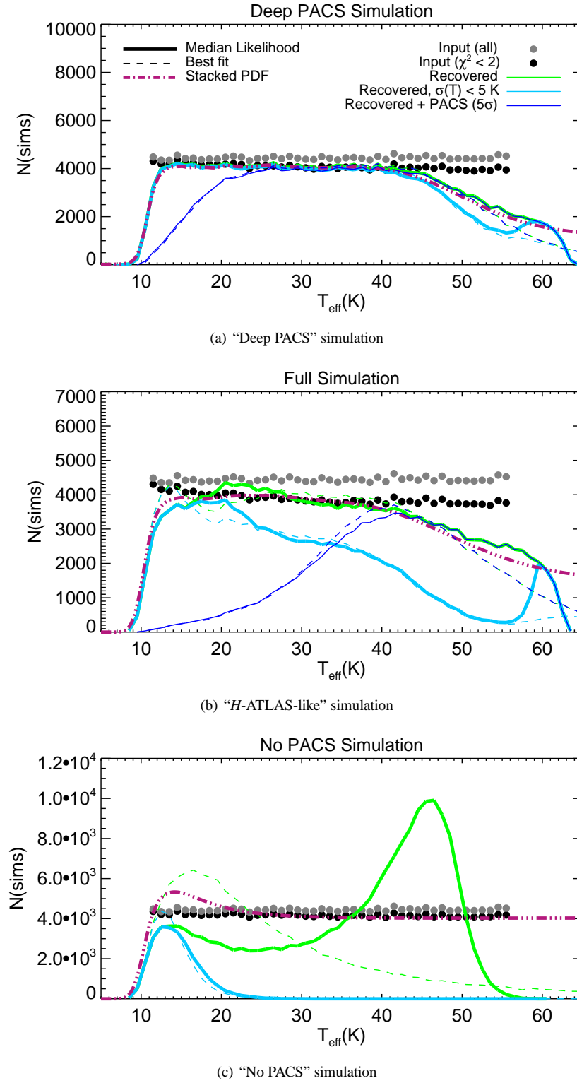
Figure 13. Histograms showing the input and output values of T_{\text{eff}} in our fixed \beta = 1.82 simulations, “Deep PACS”, “H-ATLAS-like” and “No PACS”, from top to bottom, respectively, with the input values (i.e. true temperatures) indicated by grey circles. The distribution of input temperatures for the sources for which we derive good fits is shown in black, and the output results (i.e. the values recovered by our fitting, with no SNR cuts apart from the 250\ \mu\text{m} selection criterion) for the same set of galaxies is in green, allowing the two to be directly compared. We also include the distribution of the subsample of galaxies with good fits and good temperature constraints (i.e. \sigma(T_{\text{eff}}) < 5\ \text{K} ) in light blue. The histogram of recovered values for sources with > 5\sigma PACS detections is shown by the darker blue lines (“recovered + PACS” in the legend). The median-likelihood recovered values are indicated by the solid lines, while the best-fit values are shown by the dashed lines of the same colour scheme, while the purple dot-dot-dashed lines show the renormalised stacked temperature PDF for all the galaxies with good fits ( \chi^2 < 2.0 ).
