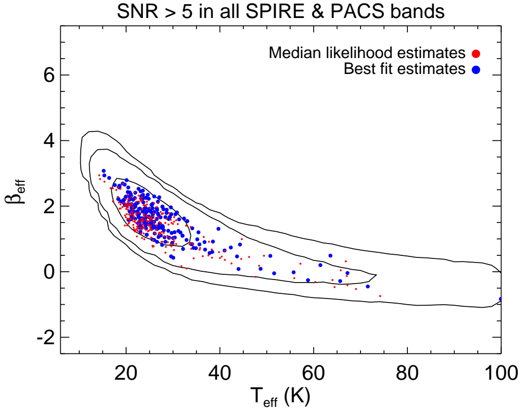
Figure 2. The relationship between T_{\text{eff}} and \beta_{\text{eff}} for only those 238 sources with the best photometry in H -ATLAS, with the best-fit (blue) and medium-likelihood (red) values overlaid on the 68.3, 95.5, and 99.7 per cent confidence contours (i.e. equivalent to the 1, 2, and 3\sigma levels assuming Gaussian statistics, in black).
