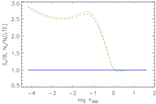
Fig. 7. The ratio of the line source function with the Planck function S_l/B_\lambda(T) for the two cases x = 1.0 (dashed lines) and x = 0.0 (dotted lines) in a metal-poor ( [\text{Fe}/\text{H}] = -3.0 ) Sun, see text for details. Also shown are the departure coefficients \beta = N_l/N_l^{\text{LTE}} for the lower level of the OH transition for x = 1.0 and x = 0.0 (solid lines), emphasizing that the non-LTE effect is purely due to scattering and not changes in the line opacity
