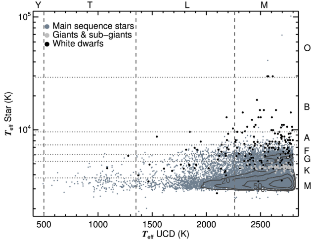
Figure 2. The distribution of secondary versus primary T_{\text{eff}} for our simulated CGB population. Spectral type divisions are indicated along the top and right axis. Different primary types are plotted in different shades (dark grey, light grey and black for main-sequence, sub-giant and white dwarfs respectively). We overplot density contours over the main sequence samples to show the structure of the distribution in highly crowded regions. Contour labels are, from the outermost to the innermost, 10, 20, 50, and 100 objects per 25 \times 100 \text{K}^2 bin.
