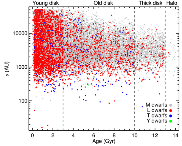
Figure 3. The projected separation s versus age distribution of our simulated CGBs. UCD spectral types are coloured as in Figure 1
