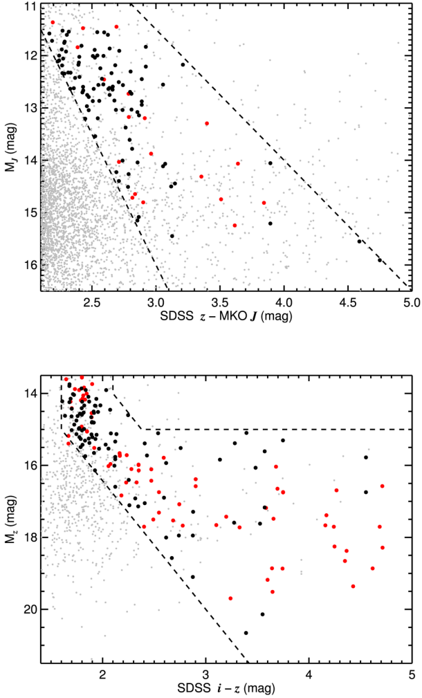
Figure 10. The colour-magnitude diagrams used to select our benchmark candidates. In each plot the selection region is enclosed by dashed lines, with good candidates plotted in black and rejected objects (considering both diagrams) plotted in gray. Red filled circles indicate known UCDs (with measured parallaxes) that were used to guide the selection criteria.
