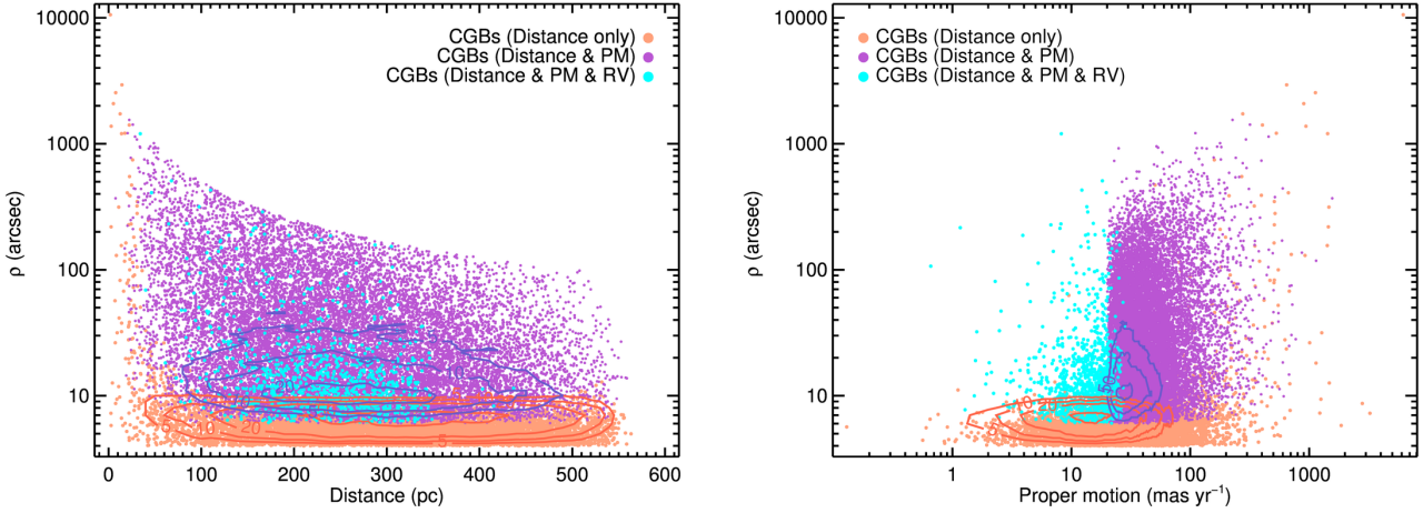
Figure 9. Angular separation ( \rho ) versus distance (left panel), and \rho versus total proper motion (right panel) for the CGBs. Benchmarks that acquired CGB status (i.e. false-alarm-probability < 0.0001 ) based only on common-distance mimics are shown in orange. Those that acquired CGB status based on common-distance and common-proper motion mimics are shown in purple. And those that also required common-RV assessment are shown in cyan. We overplot density contours over the “distance only” and the “distance & PM” samples to show the structure of the distribution in highly crowded regions. Contour labels are 5, 10, 20, and 50 objects per 10 \text{ pc} \times 1 \text{ arcsec} bin in the left panel, and objects per 1 \text{ mas yr}^{-1} \times 1 \text{ arcsec} bin in the right panel.
