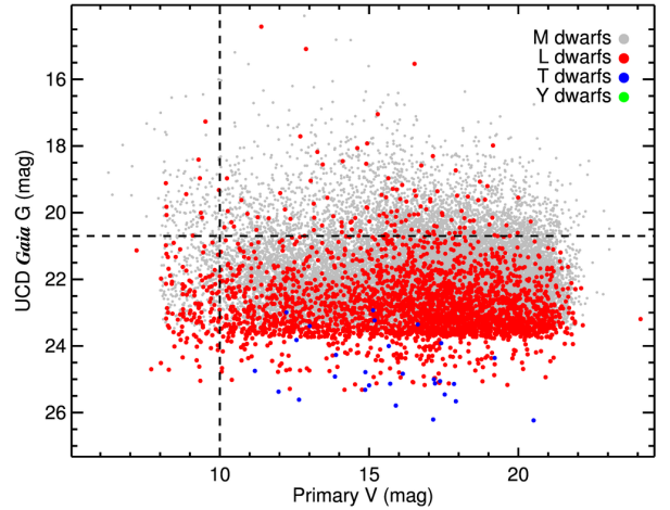
Figure 6. The Gaia G -band magnitudes of CGBs versus V -band primary magnitudes, with UCD spectral types coloured as in Figure 1. Dashed lines indicate the Hipparcos limit ( V \sim 10 mag) for the primaries, and the Gaia G detection limit for the CGBs.
