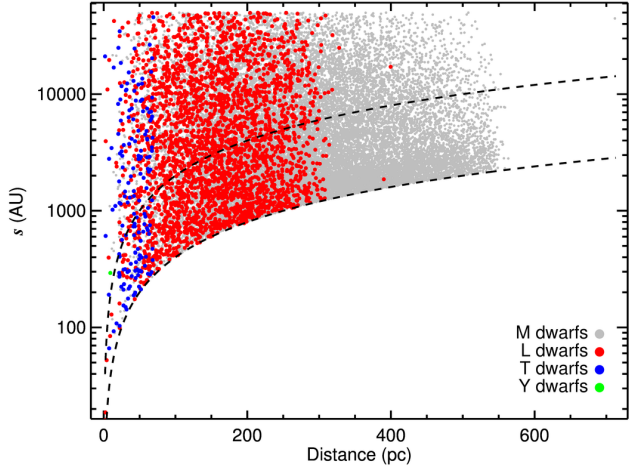
Figure 4. The projected separation versus distance distribution of our simulated CGBs. UCD spectral types are coloured as in Figure 1. The two dotted lines represent the 4 arcsec and 20 arcsec limits (see section 2.3).
