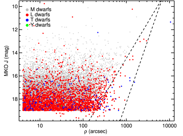
Figure 7. J -band magnitude versus angular separation ( \rho ) for our simulated CGBs, with UCD spectral types coloured as in Figure 1. At wide separation increased false alarm probability leads to truncation in the CGB population (see Section 3.2.2), with hard cut-offs (for the M and L systems) shown by dashed lines.
