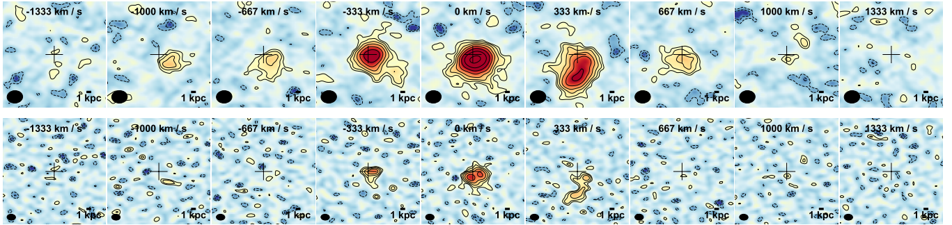
Figure 3. CO J(2\rightarrow 1) maps of SDSS J1341–0321 averaged over 333 \text{ km s}^{-1} channels spanning \Delta V = \pm 1500 \text{ km s}^{-1} (labels give channel centers) relative to the systemic redshift. The top row shows the naturally weighted images and the bottom row shows the Briggs ( R = 0 ) weighted images. Contours start at 2\sigma and are logarithmically spaced at 0.2 dex multiples of \sigma . Dashed contours are negative equivalents. The crosshair indicates the peak of the stellar emission in the HST /F814W imaging (Figure 1). Black ellipses show the FWHM of the synthesized beam.
