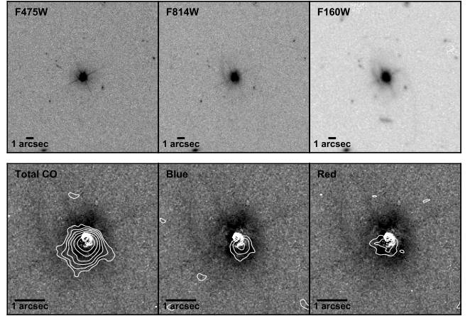
Figure 1. (top) HST WFC3 UVIS (F475W, F814W) and IR (F160W) images of SDSS J1341–0321 spanning 20'' . Two faint tidal tails are visible and extend over several arcseconds ( 1'' \approx 7 kpc), but the majority of the stellar emission is unresolved. (bottom) 5'' zoom-ins showing the Sérsic model-subtracted F814W image (section 3.2) as greyscale and CO J(2 \rightarrow 1) contours, averaged over (left) |\Delta V| < 1000 \text{ km s}^{-1} , (middle) -1000 < \Delta V < -500 \text{ km s}^{-1} , (right) 500 < \Delta V < 1000 \text{ km s}^{-1} . CO J(2 \rightarrow 1) contours start at 3\sigma and are logarithmically spaced at 0.2 dex multiples of \sigma . All images are orientated north up, east left. Note that the absolute astrometric precision of the HST images (boresight-aligned to SDSS) is \delta_\theta \approx 0.2'' .
