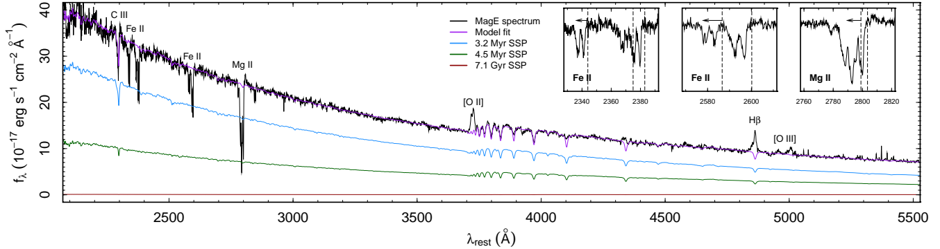
Figure 2. Magellan Echellette (MagE) optical spectrum of SDSS J1341–0321 in the rest-frame. We show the best fitting model from our SSP modelling (Section 3.2) illustrating that the stellar continuum emission is dominated by very young ( t < 5 Myr) populations. The redshift z = 0.6611 is determined from the stellar absorption lines. The inset panels show zoom-ins of the model continuum normalized spectrum around the Fe II \lambda\lambda 2344, 2374, 2383, 2587 & 2600\text{\AA} and Mg II \lambda\lambda 2796, 2804\text{\AA} ISM absorption lines. Vertical dashed lines indicate the rest-frame wavelengths of the lines, and the arrows indicate a blueshift vector of -1000\text{ km s}^{-1} . Note that the 7.1 Gyr component is so weak relative to the young populations it appears almost featureless in this plot.
