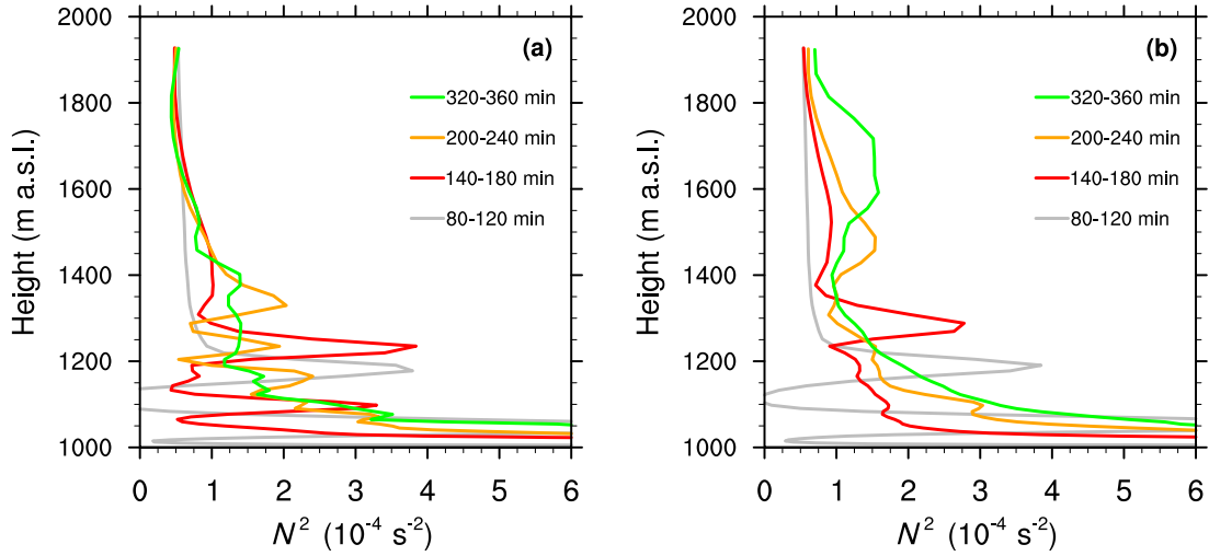
Figure III.9: Vertical profiles of the Brunt-Väisälä frequency N^2 , averaged over the x and y ranges of the valley centre and over time intervals of 40 min for the 3D (a) and 2D (b) valleys.
