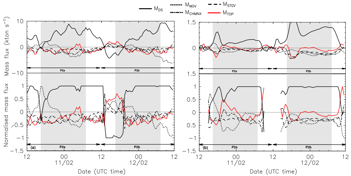
Figure V.10: Timeseries of the mass fluxes through DS ( M_{DS} ), MGV ( M_{MGV} ), CHMNX ( M_{CHMNX} ), STGV ( M_{STGV} ), vertically integrated from the ground surface to z = z_m , and through the top surface at z = z_m ( M_{TOP} ) for the period from 10 February 2015 at 1200 UTC to 12 February 2015 at 1200 UTC in WRF-R (a) and WRF-I (b); see Fig. V.1b and V.1c for the location of the gates. The nighttime periods (from sunset to sunrise) are displayed as grey shading. The bottom panel shows the mass fluxes normalised by the total mass flux out of the Passy Valley. Positive and negative values of the mass flux correspond to a flux out of and into the Passy Valley, respectively.
