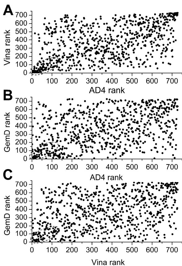
Figure 3: Correlation between the ranking of molecules in the DUD dataset for the target RXRa. The rank obtained with one docking algorithm was plotted against the rank obtained with another algorithm. The area surrounded by a dashed line highlights some correlation observed at the highest ranking ligands. A) AutoDock Vina ranks plotted against AutoDock ranks, B) GemDock ranks plotted against AutoDock ranks and C) GemDock ranks plotted against AutoDock Vina ranks.
