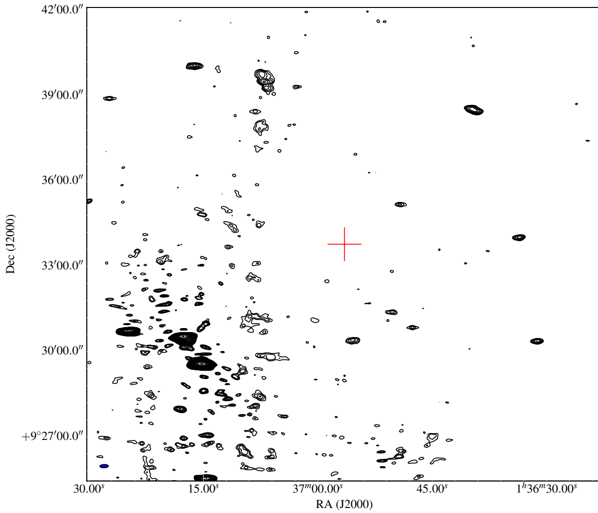
Figure A3. The field around SIMP0136. As Figure A1, but the rms noise at this position is 220 \mu\text{Jy beam}^{-1} and the resolution 16.1 \times 6.7 arcsec. In the SE of the image dynamic range limitation around the bright source 4C +09.06 (4.7 Jy) can be seen.
