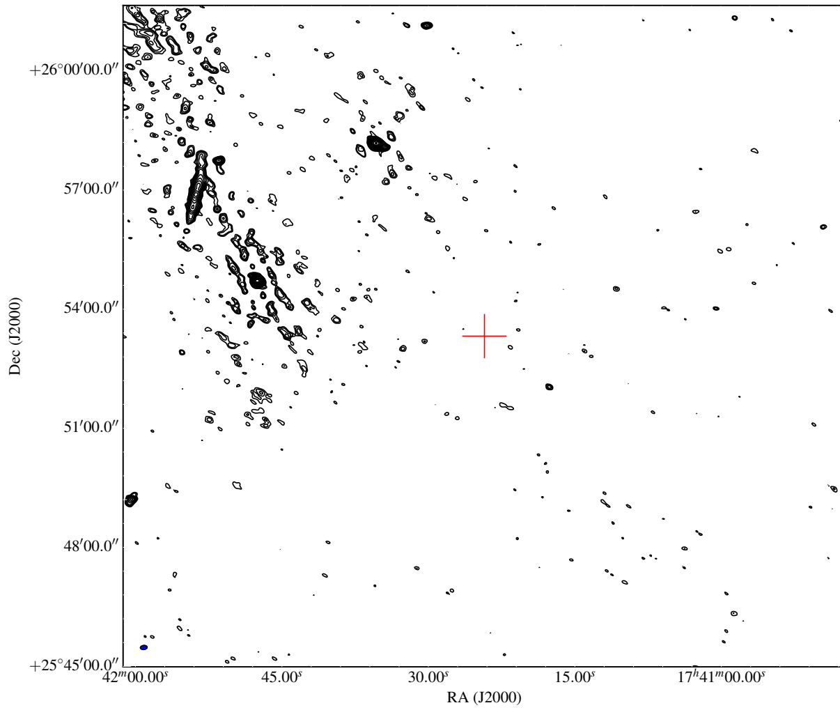
Figure A2. The field around WISE1741. As Figure A1, but the rms noise at this position is 290 \mu\text{Jy beam}^{-1} and the resolution 9.4 \times 6.3 arcsec. The extended source referred to in the text can be seen to the NE.
