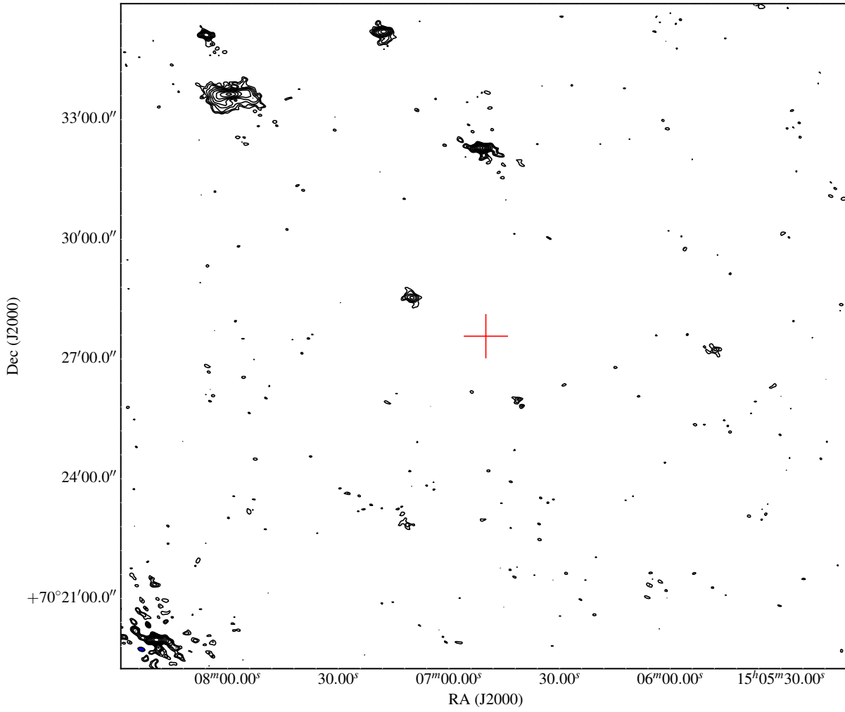
Figure A1. The field around WISE1506. A red cross marks the position of the target. Rms noise at this position is 240 \mu\text{Jy beam}^{-1} ; contours are at 3 \times 240 \times (1, \sqrt{2}, 2, \dots) \mu\text{Jy beam} . The resolution of the image is 9.3 \times 5.5 arcsec, shown by a blue ellipse in the bottom left-hand corner.
