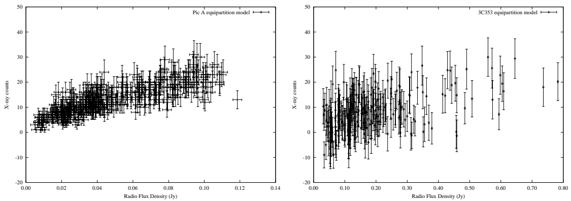
Figure 4.7: Examples of the linearly-scale model simulated X-ray counts against radio flux density for Pic A (left panel) and 3C 353 (right panel).
