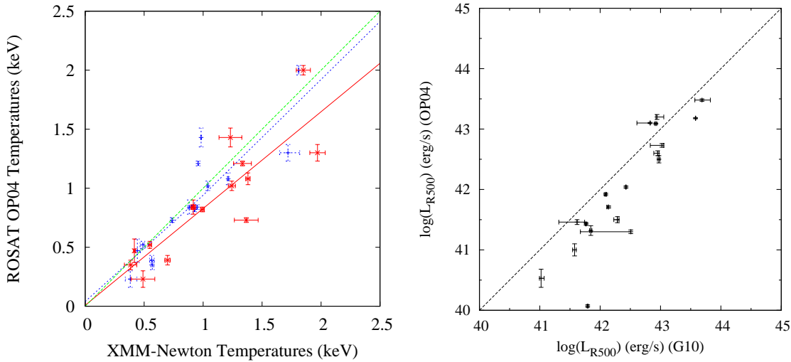
Figure 6.5: Comparison between these XMM-Newton temperatures (left panel) and luminosities (right panel) and the ROSAT results by Osmond & Ponman (2004). In the temperature comparison, the spectral temperatures are shown in blue, and the profile temperatures in red with the corresponding regression line fits plotted in the same colours. The green line is a line of equality.
