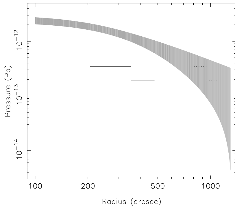
Figure 3.11: Pressure profile for the northern sub-cluster shown by the greyed in region, with the measured pressure of the lobes of 3C 353 at the projected distance (solid line) and at the position with the radial shift applied to where the East lobe is in pressure balance with the sub-cluster (dashed line). The measured iC emission was used to determine the pressure within each lobe. The temperature of the cluster at the radial distance of 3C 353 was used.
