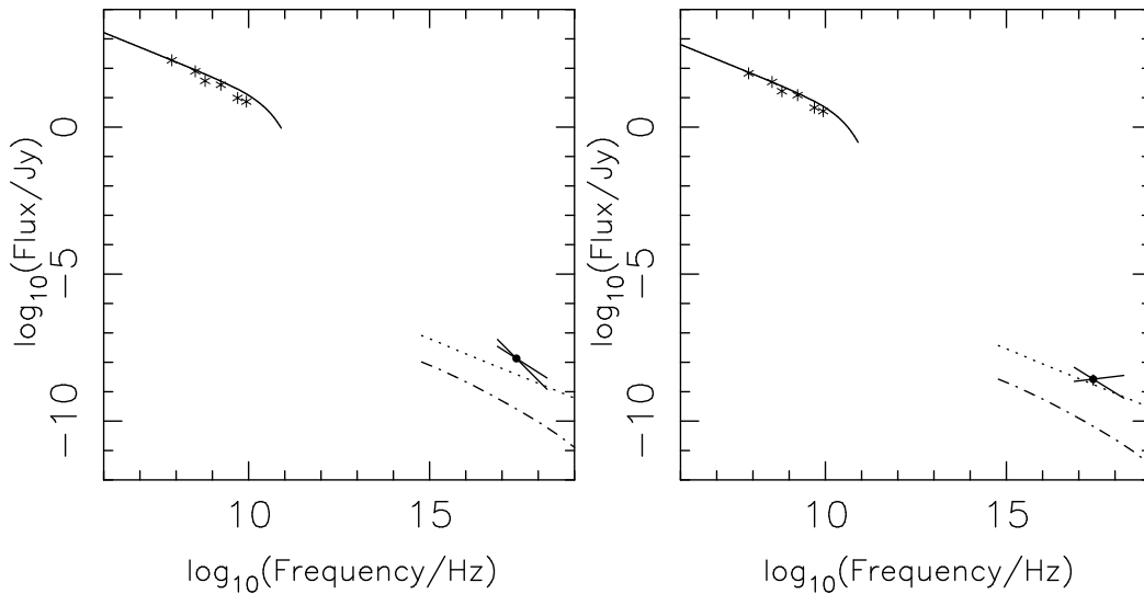
Figure 3.8: Broad-band spectrum for the East (left) and West (right) lobes of 3C 353 . A synchrotron emission model (solid line) is fitted to the radio data (asterisks). The measured X-ray flux is represented by the dot with the bowtie indicating the error. The dotted line shows the iC X-ray flux prediction and the dash-dotted line shows the predicted synchrotron self-Compton emission, both with the equipartition magnetic field strength.
