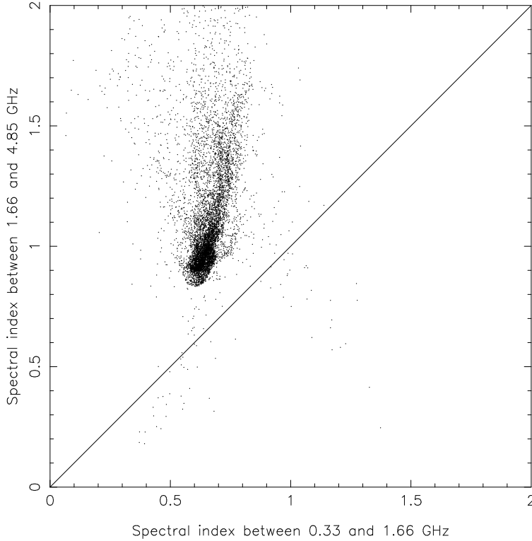
Figure 3.10: Colour-colour diagram for 3C 353 made at 7 arcsec resolution.
