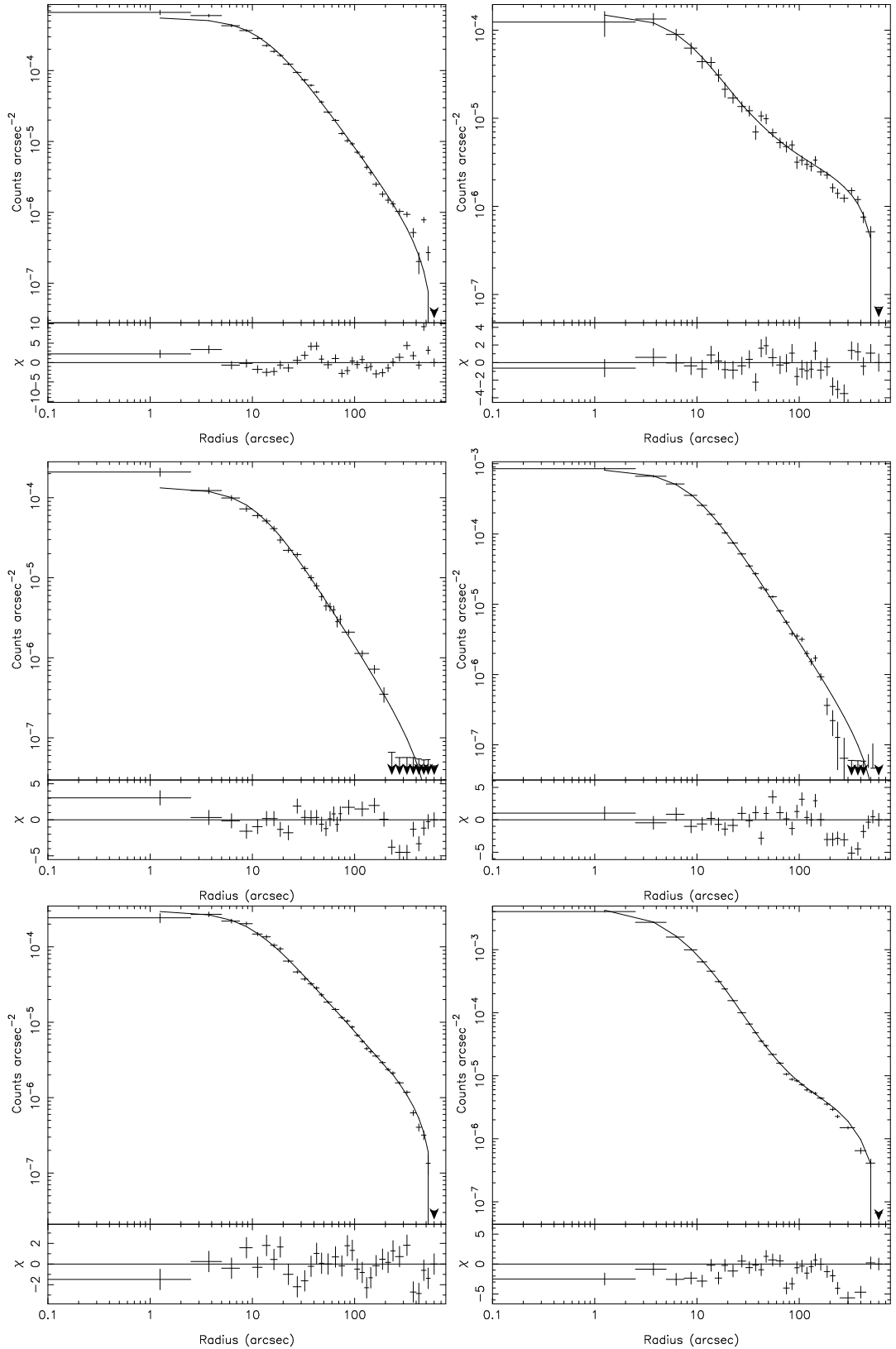
Figure 6.4 continued. From left to right are the surface brightness profiles of NGC 1407 and NGC 3607 on the top row, NGC 3665 and NGC 3923 on the middle row, and NGC 4073 and NGC 4261 on the bottom row.
