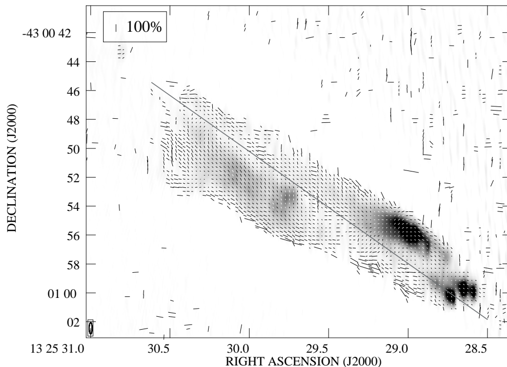
Figure 5.10: Radio polarisation in the inner jet of Cen A showing the direction of the magnetic field vectors on a composite, Stokes I, 8.4 GHz radio map. The radio image is in the range 0.1 – 0.01 Jy and a vector 0.56 arcsec long represents 100%. The solid grey line highlights a possible axis of null polarisation discussed in Section 5.3.5.
