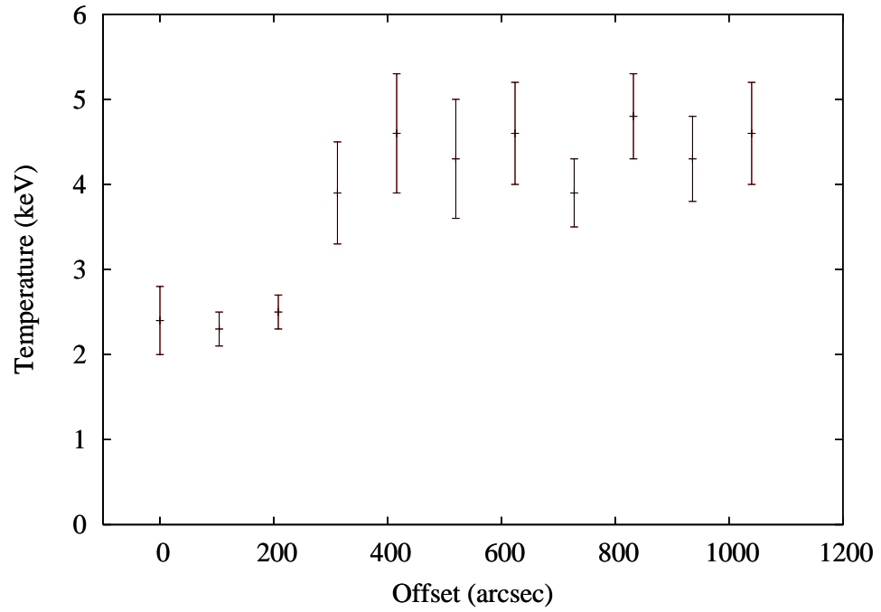
Figure 3.5: Temperature variation of north-south slice through cluster with rectangular regions of 208 \times 104 arcsec from a zero of offset at 17:20:50.074, -00:53:13.77.
