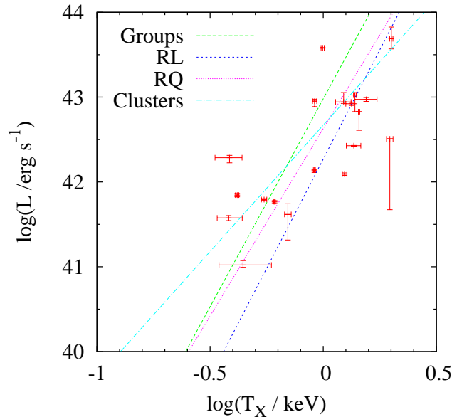
Figure 6.9: Temperature-Luminosity relationships for all the groups using the truncated, weighted-mean temperatures ( T_p ) and the Bayesian estimated luminosity. The relationship for clusters (Equation 6.2) is shown with the cyan dashed-dotted line, Equation 6.3 for groups is shown with the green long-dashed line, the relationship for radio-loud groups (Equation 6.4) is shown with the blue dashed line and the relationship for radio-quiet groups (Equation 6.5) is shown in the magenta dotted line.
