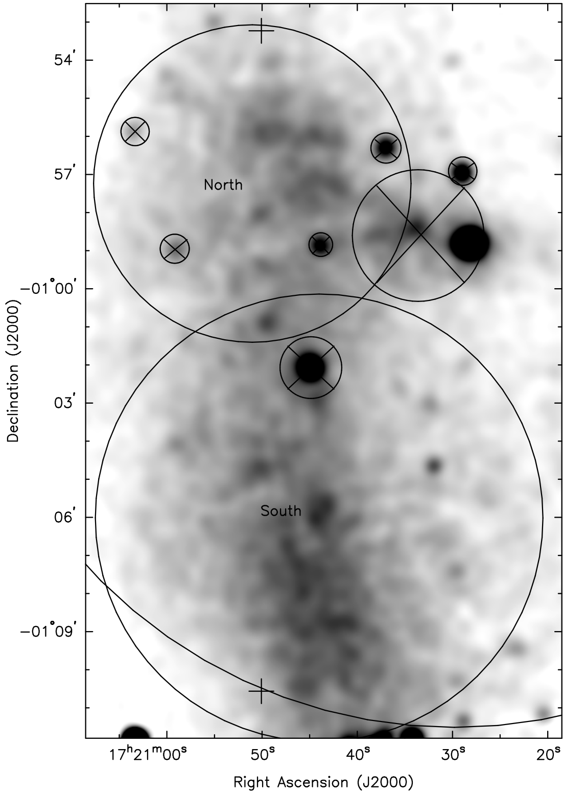
Figure 3.4: Northern and southern sub-cluster regions from which spectra were extracted to determine the sub-cluster global temperatures. The crossed regions are those which were excluded from the analysis and include the X-ray point sources and 3C 353. The crosses indicate the limits of the slice used. The inner edge of a large annular region masking the edge of the camera can be seen at the bottom of the image.
