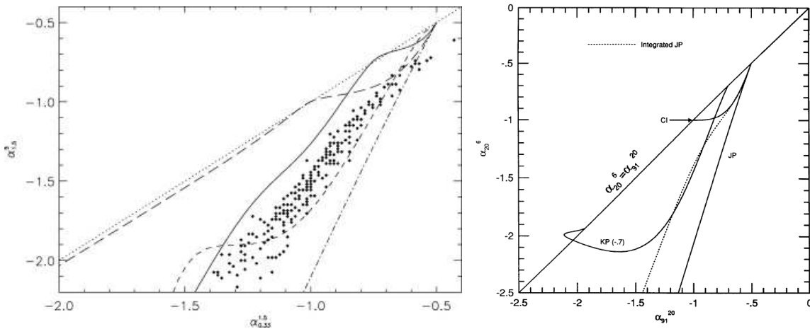
Figure 4.9: Colour-colour diagrams showing the conventional spectral ageing model predictions for the leaky box model with various diffusion rates indicated by the difference line styles (Kaiser 2005) with the observational data for Cygnus A from Rudnick et al. (1994) (left panel) and the standard KP, JP and continuous injection (CI) models taken from Katz-Stone et al. (1993) (right panel).
