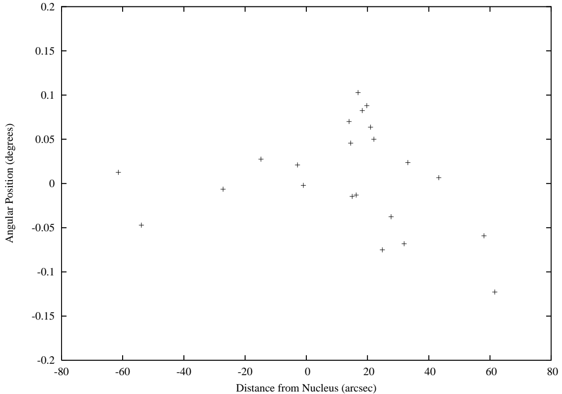
Figure 5.4: The offset between the position angle of the jet in Cen A ( 54^\circ ) and the transverse position of the radio knots as a function of the projected distance from the nucleus for the knots in the jet and counterjet (negative distances). The knots do not appear to lie at the PA 54^\circ for the entire length of the jet.
