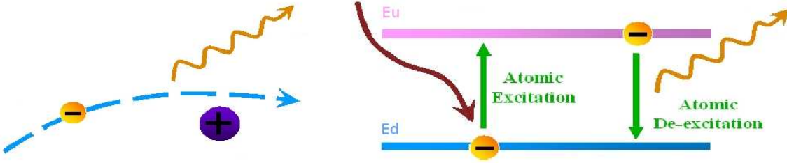
Figure 1.3: Diagrams of the bremsstrahlung emission mechanism (left) and line-excitation and de-excitation (right). As in Figure 1.1, in the left panel the path of the electron is shown by the dashed cyan line, the incident low-energy photons is shown by the red wave and the higher-energy X-ray photon by the orange wave. In the right panel, the movement of the electron between the upper energy level (pink) and the lower energy level (cyan) is shown by the green lines.
