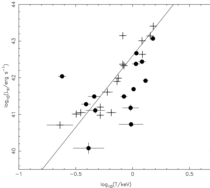
Figure 6.8: Temperature-Luminosity relationships for the original group sample using ROSAT data (Croston et al. 2005a, Figure 2, bottom panel). The plus symbols are the radio-quiet groups and the filled circles are the radio-loud groups with the best fitting radio-quiet relationship, overplotted.
