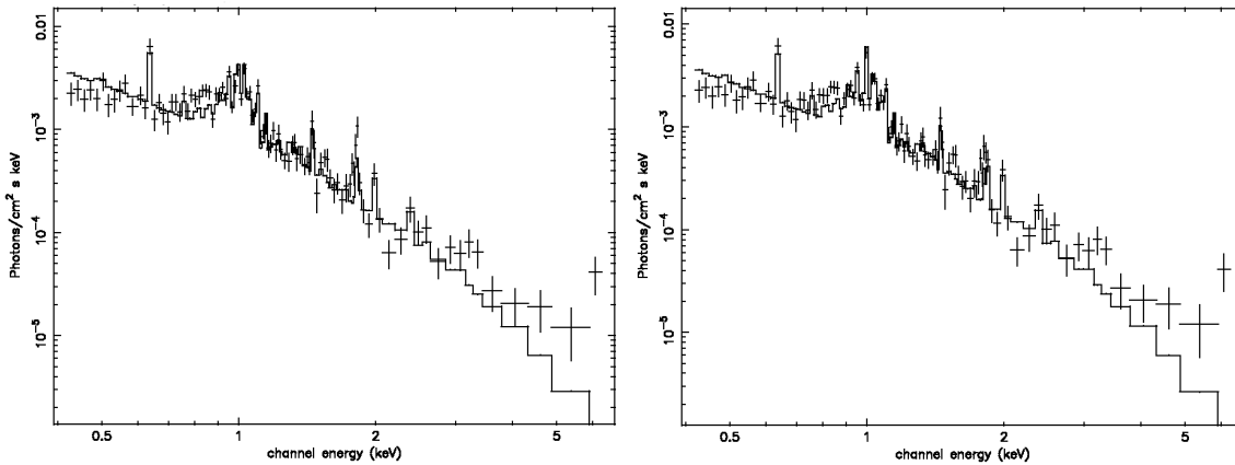
Figure 1.4: Thermal predictions for X-ray emission using the mekal model (left panel) and the apec model (right panel). The data plotted is the MOS1 Chandra data for NGC 533. The temperature of the hot gas in this group is \sim 1.21 keV, with a fixed Galactic absorption of n_H = 3.01 \times 10^{20} \text{ cm}^{-1} and a redshift of z = 0.0181 .
