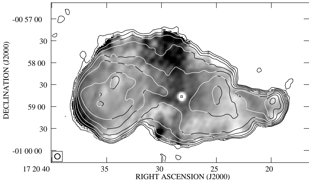
Figure 3.9: Spectral index map between 1.67 GHz and 327 MHz with radio contours at 327 MHz for levels of 0.01 \times (1, 2, 4, \dots) mJy/beam. The beam size (7.0 arcsec) is shown by the circle in the bottom left corner.
