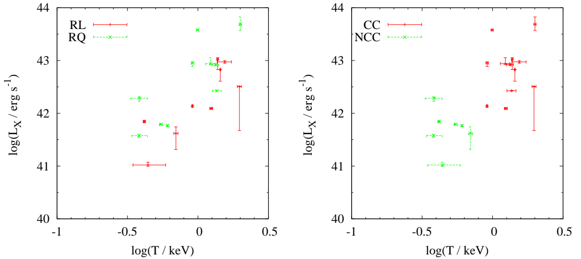
Figure 6.11: Temperature-Luminosity relationships for the radio-loud groups (red solid lines) and radio-quiet groups (green dashed lines) in the left panel and the cool-core groups (red solid lines) and non cool-core groups (green dashed lines) in the right panel as defined from our temperature profiles (Figure 6.2). NGC 1052 is not included in the CC/NCC comparison as its bright core prevents us from measuring its temperature profile.
