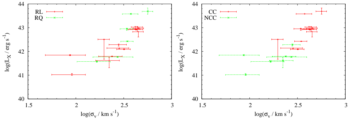
Figure 6.14: Luminosity- \sigma_v relationships for radio-loud (red) and radio-quiet (green) groups in the left panel and CC (red) and NCC (green) in the right panel.
