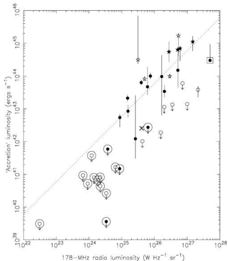
Figure 3.7: X-ray luminosity of the accretion-related component as a function of 178-MHz total radio luminosity for LERGs (open circles), NLRGs (filled circles), BLRGs (open stars) and quasars (filled stars) as presented in Hardcastle et al. (2006b) with the position 3C 353 indicated by the cross.
