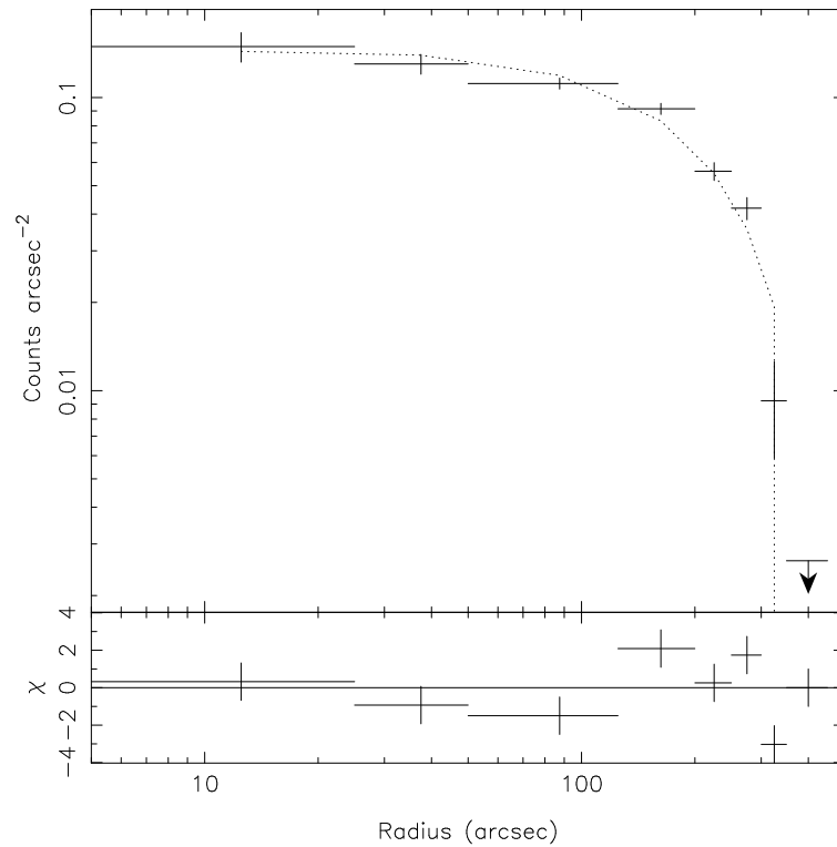
Figure 3.6: Surface brightness profile for the northern sub-cluster showing the PN dataset with the best fitting \beta model which has \beta = 0.35 and core radius 194 arcsec.
