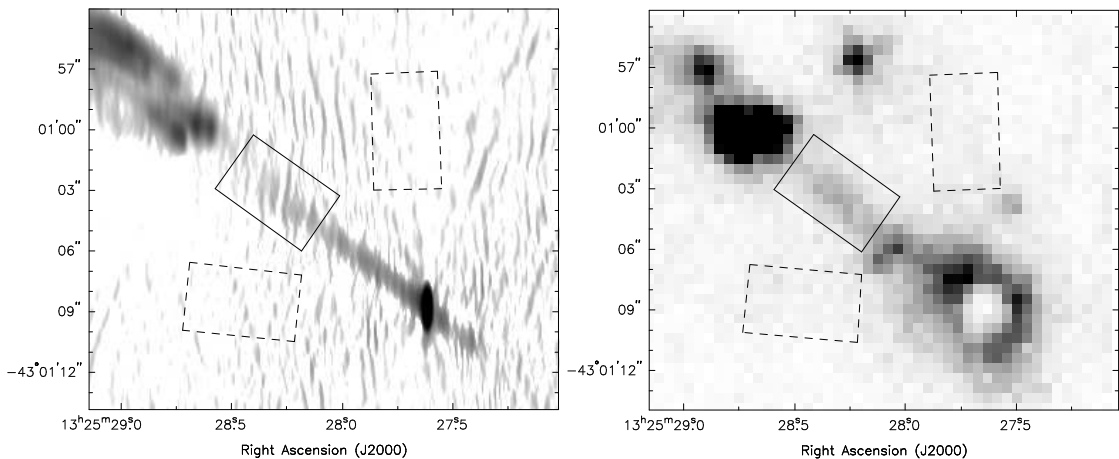
Figure 5.17: Regions used for the analysis of the hundred-parsec-scale inner jet in Cen A (discussed in Section 5.3.9) shown against the 2007 8.4 GHz radio data (left) and the combined X-ray data in the energy band 0.4 – 2.5 keV (right). The source region is shown in solid line, and the background regions in the dashed line. These regions were chosen to include as emission from only the hundred-parsec-scale inner jet, excluding the emission from the X-ray point sources near the core.
