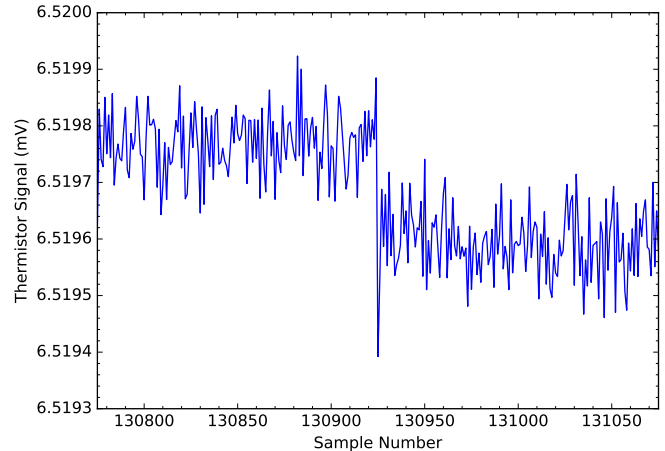
Figure 6. Example of a thermistor ‘jump’ from one of the thermistors for the 500 \mu\text{m} array, PLWT2, during ATLAS observation 1342196626.
