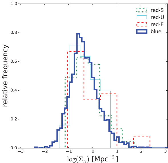
Figure 4. Distributions of the projected surface density \Sigma_5 estimated according to equation (3) in blue (thick solid line) and red sources. E (red dashed line), S (green dotted line) and U (cyan line) labels represent the morphology of individual red source. Each histogram is normalized by its integral.
