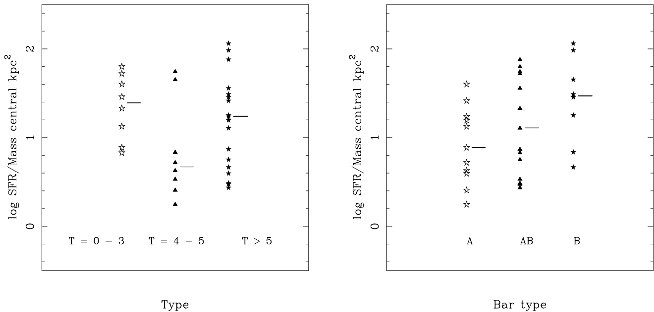
FIG. 5.—Same as Fig. 2, but for the SFR per unit stellar mass over the central kiloparsec
