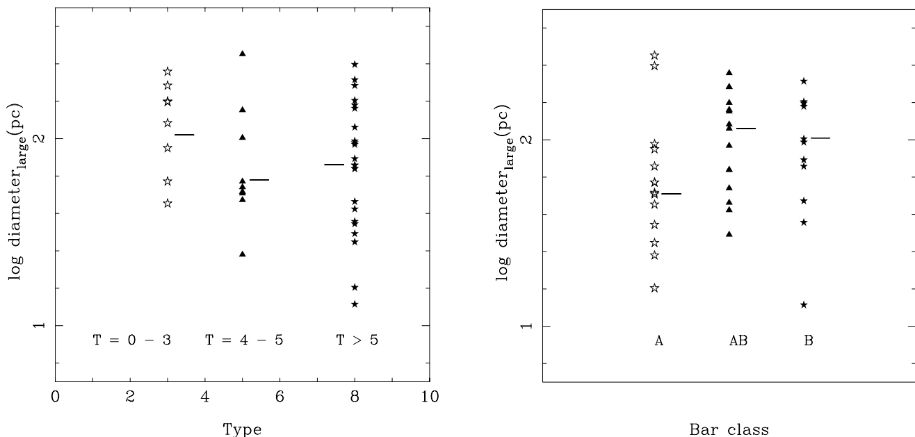
FIG. 3.—Same as Fig. 2, but for the diameter of the largest H II region
