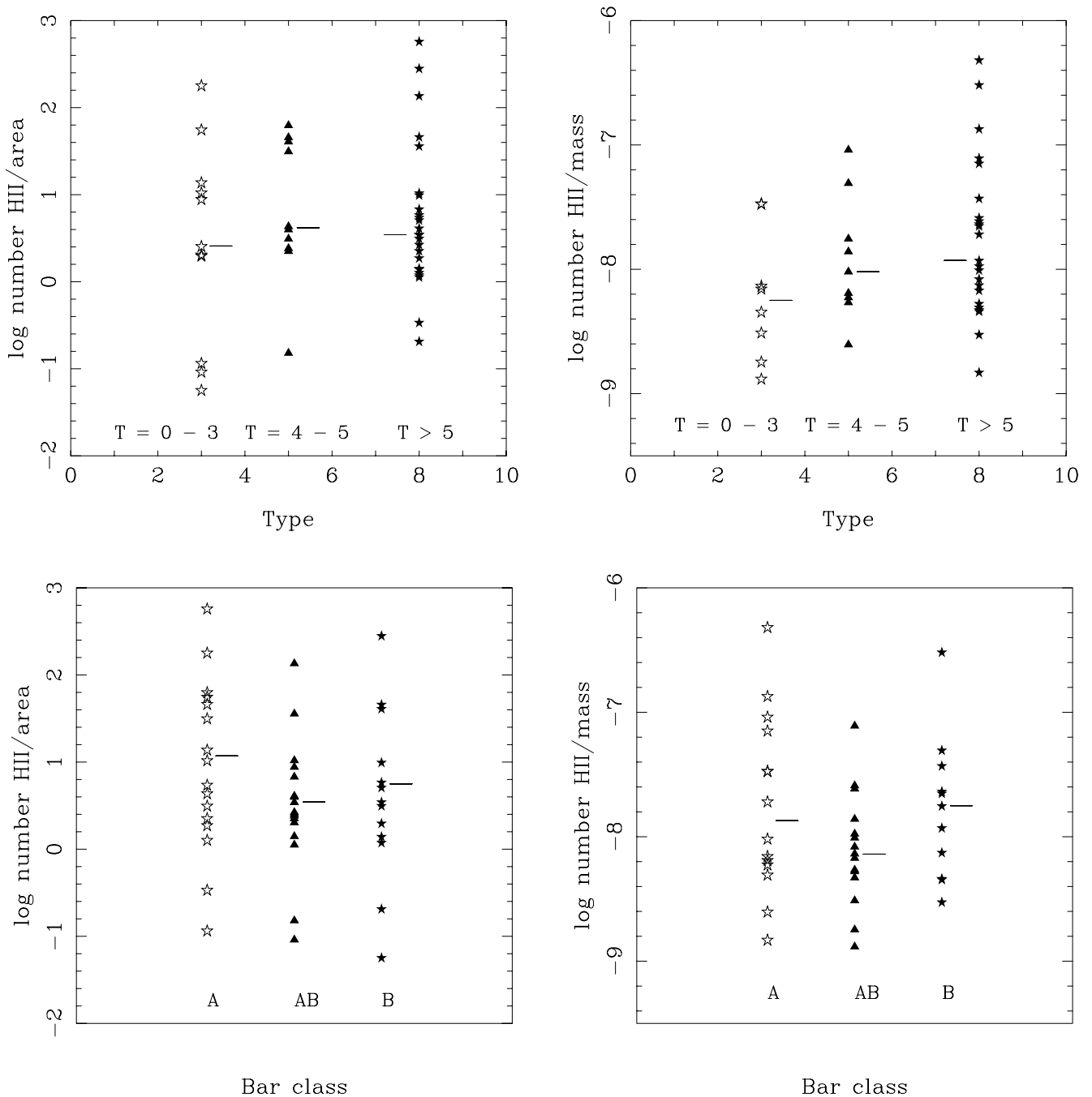
FIG. 1.— Top left : Distribution of the number of H II regions per unit area for types T = 0-3 , T = 4-5 , and T > 5 (given in Table 1). Top right : Same as left, but with number of H II regions per stellar mass unit (as traced by the H -band luminosity). Bottom : Same as top, but compared with the bar class. All diagrams are for galaxies with distances d \geq 2 Mpc. The horizontal ticks next to the symbols show the median value of the distribution.
