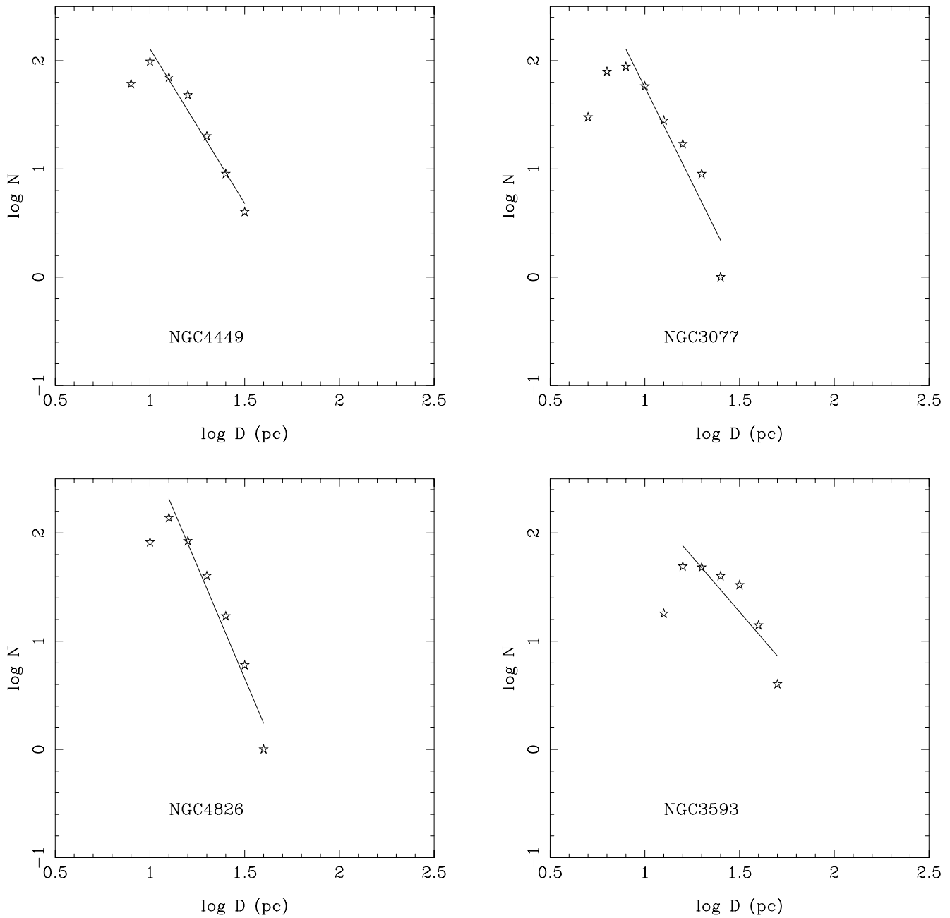
FIG. 7.—Differential diameter distributions of galaxies with 100 or more H II regions and power-law fits
