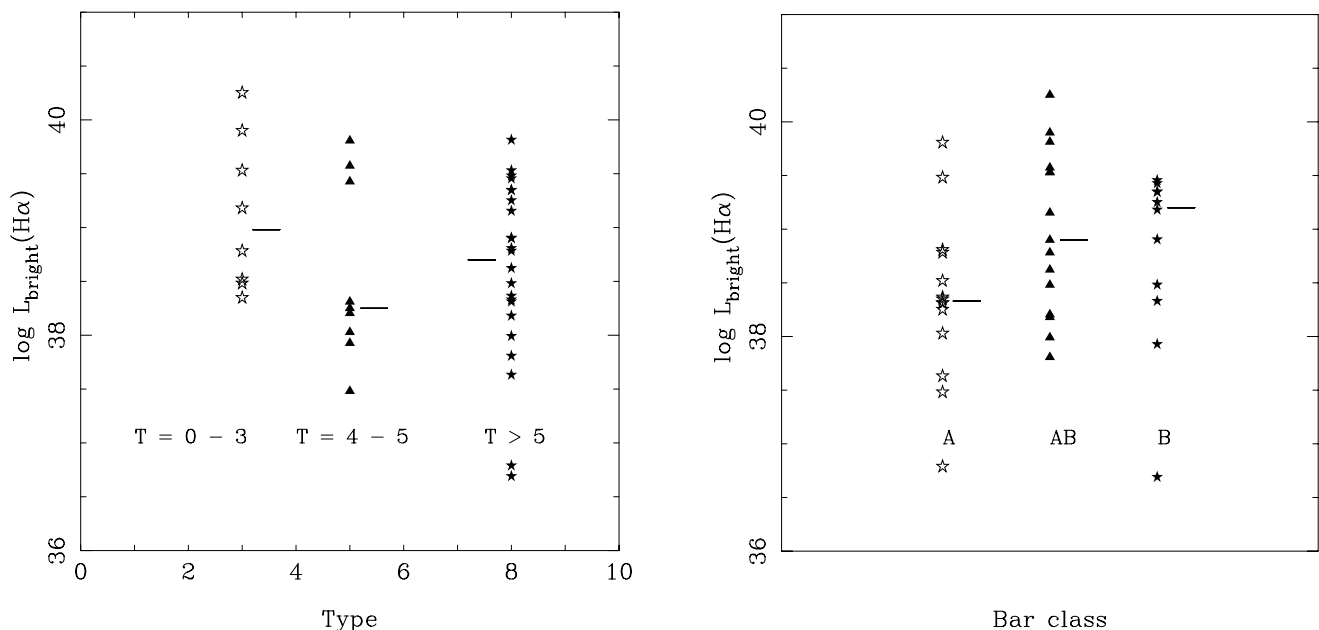
FIG. 2.—H \alpha luminosity of the brightest H II region as a function of morphological type (left) and bar class (right) for those galaxies in our sample with distances d \geq 2 Mpc.
