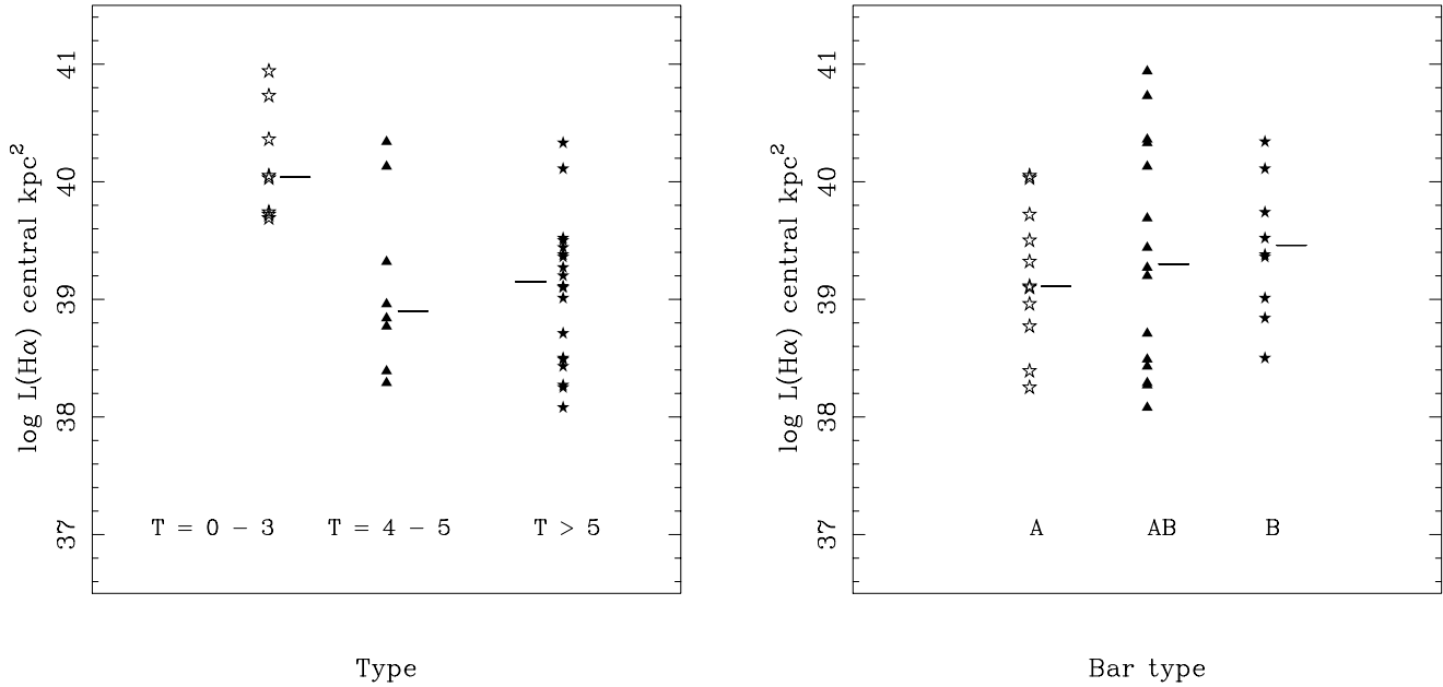
FIG. 4.—Same as Fig. 2, but for the H\alpha luminosity in H\ II regions over the central kiloparsec
