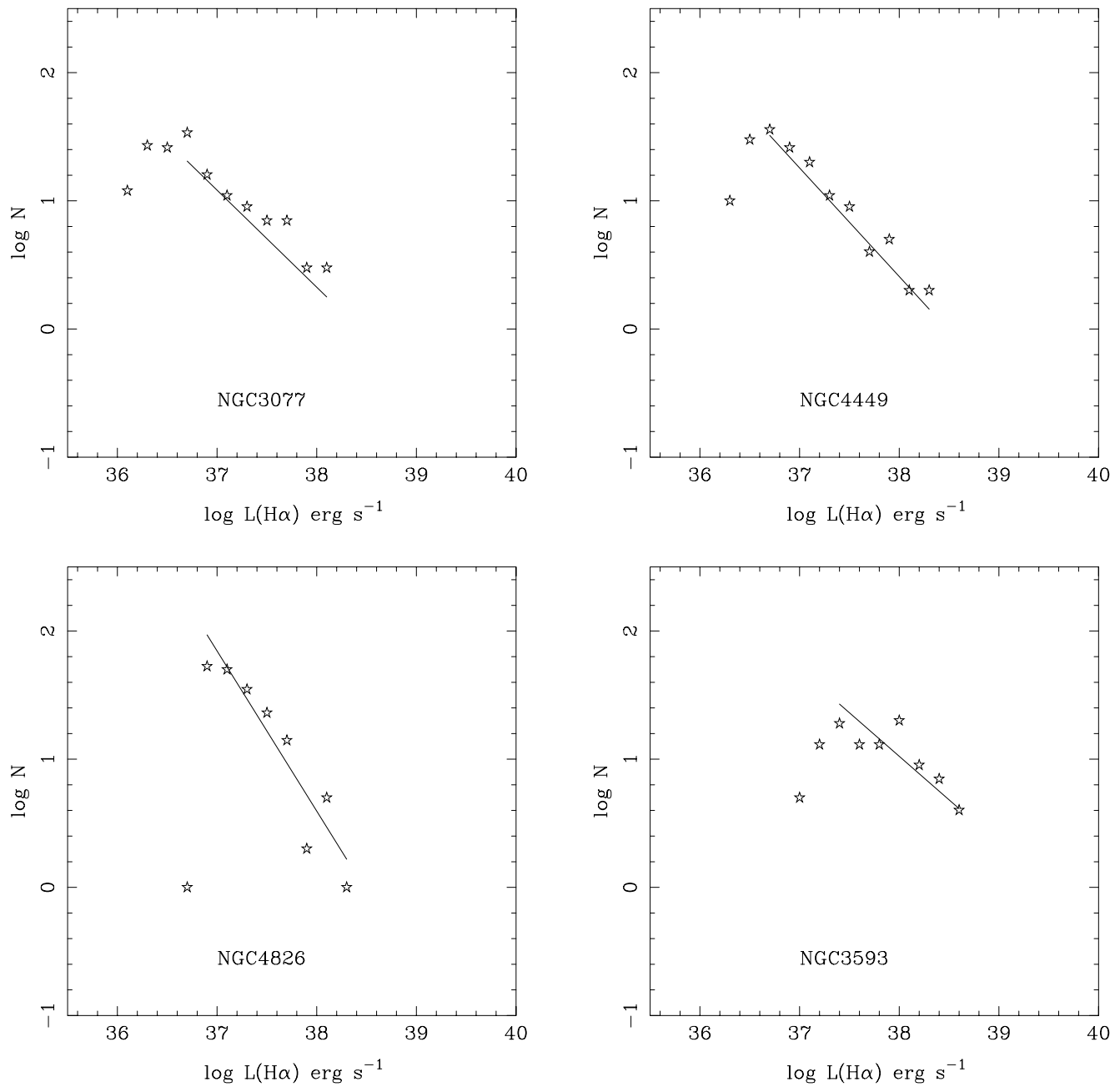
FIG. 6.—Luminosity functions of galaxies with 100 or more H II regions and power-law fits
