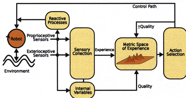
Fig. 2. Schematic of the Interaction History Architecture
