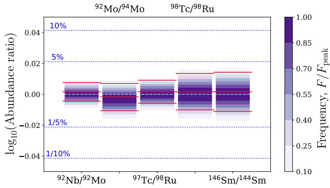
Figure 6. Same as Fig. 4 but considering only tracers in the low-density group.
