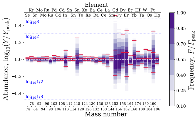
Figure 7. Same as Fig. 2 but considering only tracers in the high-density group.
