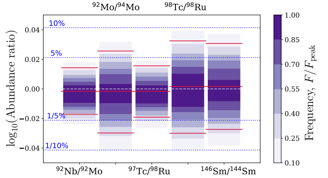
Figure 8. Same as Fig. 4 but considering only tracers in the high-density group.
