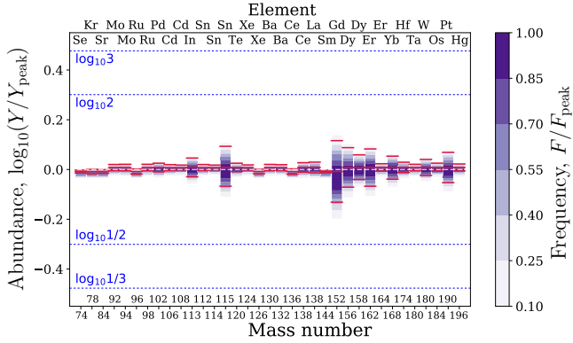
Figure 5. Same as Fig. 2 but considering only tracers in the low-density group.
