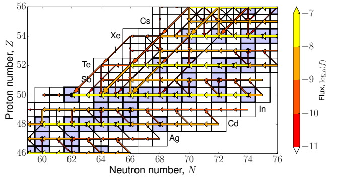
Figure 9. Integrated reaction flows in the vicinity of Sn in a trajectory of the low-density group with peak temperature 2.8 GK.
